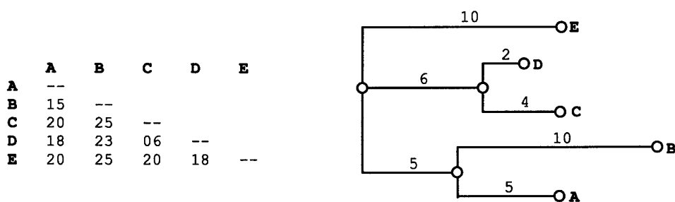
Figure 2: An example of an additive tree representation and its associated proximity matrix.
