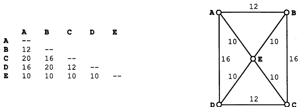
Figure 1: An example of an multidimensional scaling representation and its associated proximity matrix.
