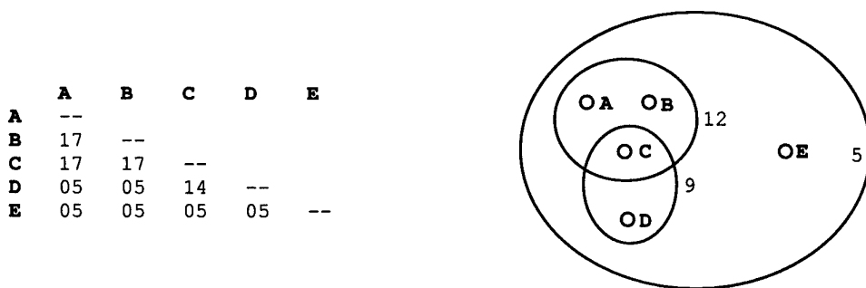
Figure 3: An example of an additive clustering representation and its associated similarity matrix.
