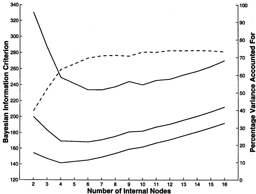
Figure 7: Bayesian Information Criterion (left hand scale, solid line) for \sigma values of 0.10, 0.15 and 0.20 (top to bottom), and Percentage of Variance Accounted For (right hand scale, broken line) values for the risk data, using additive trees with between 2 and 16 internal nodes.
