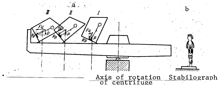
Figure 1. Diagram of arrangement of cabin on centrifuge console and forces to which man was exposed when standing on stabilographic platform (a), and diagram of distribution of weights on human body (b)
