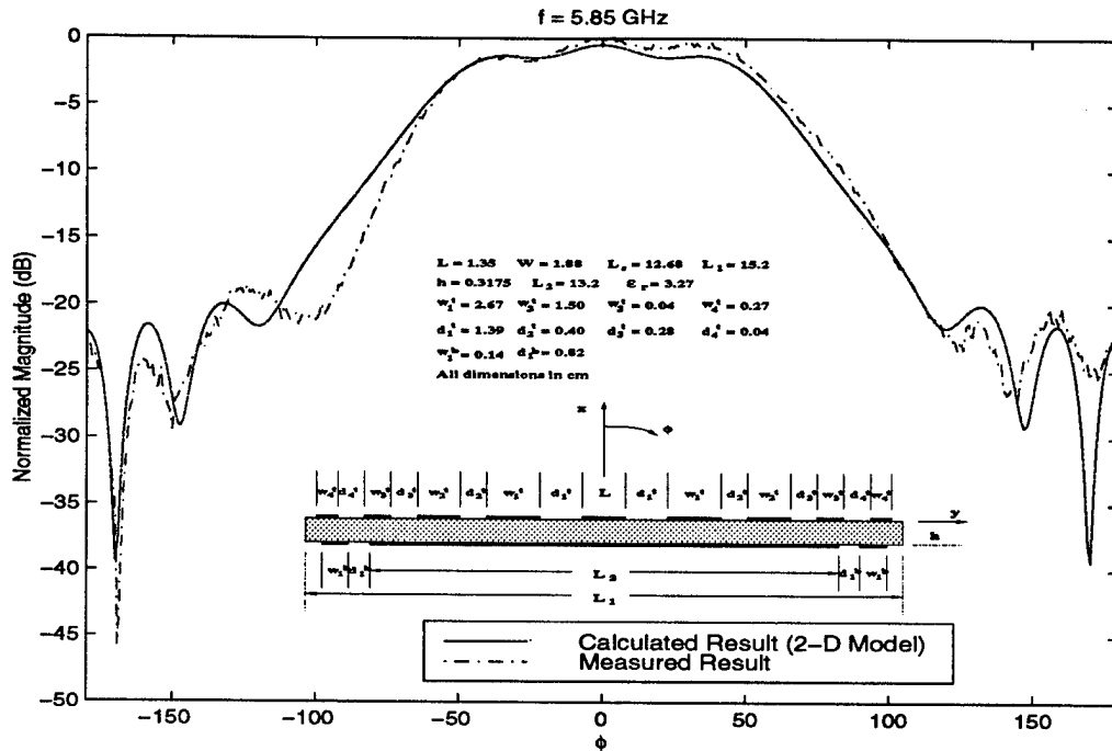
Figure 4.6: Calculated and measured result at f = 5.85 GHz
