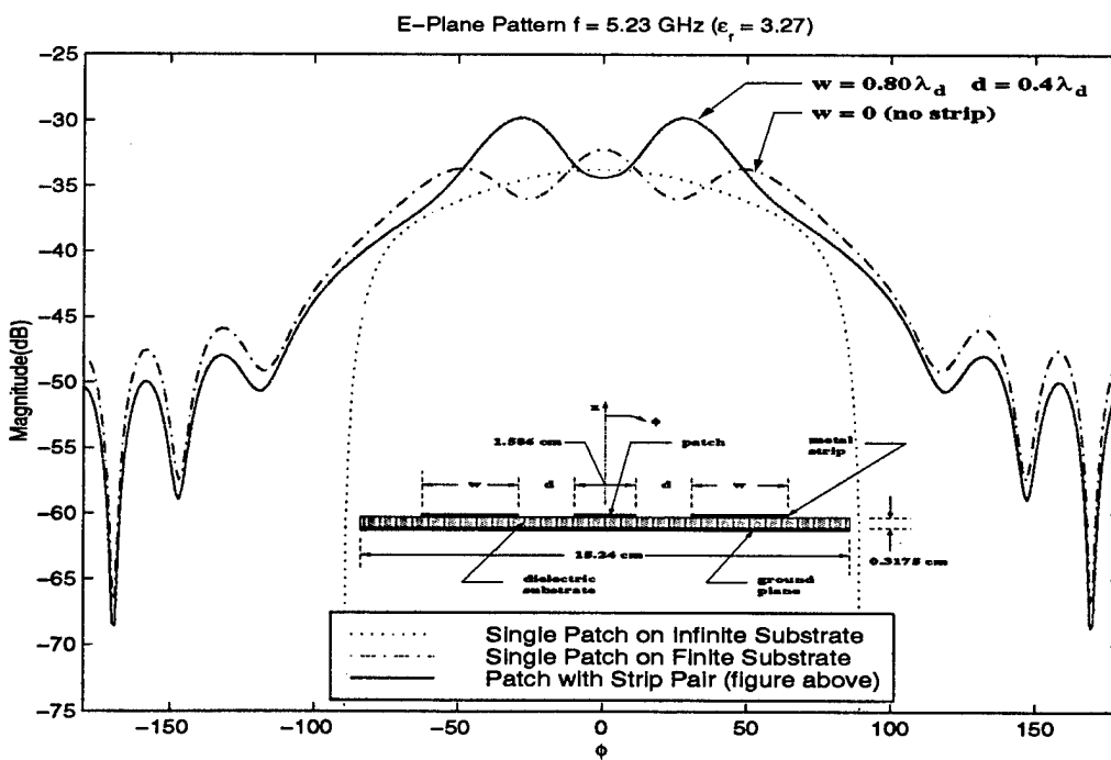
Figure 3.10: Two-strip antenna E-Plane pattern: d=0.4\lambda_d , w=0.8\lambda_d
