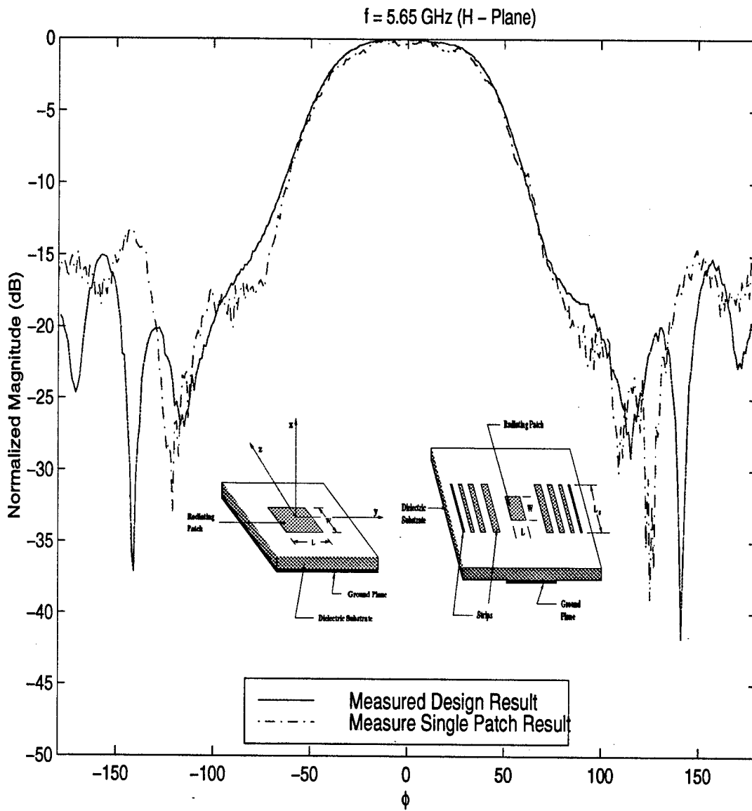
Figure 4.8: Comparison between single patch and optimal design (H-Plane)
