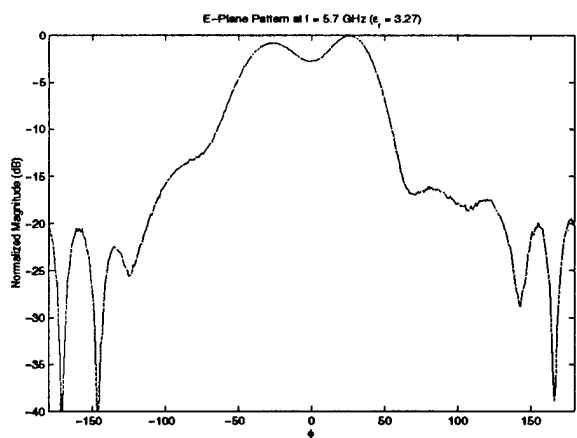
(e) E-Plane pattern at f = 5.7 GHz
