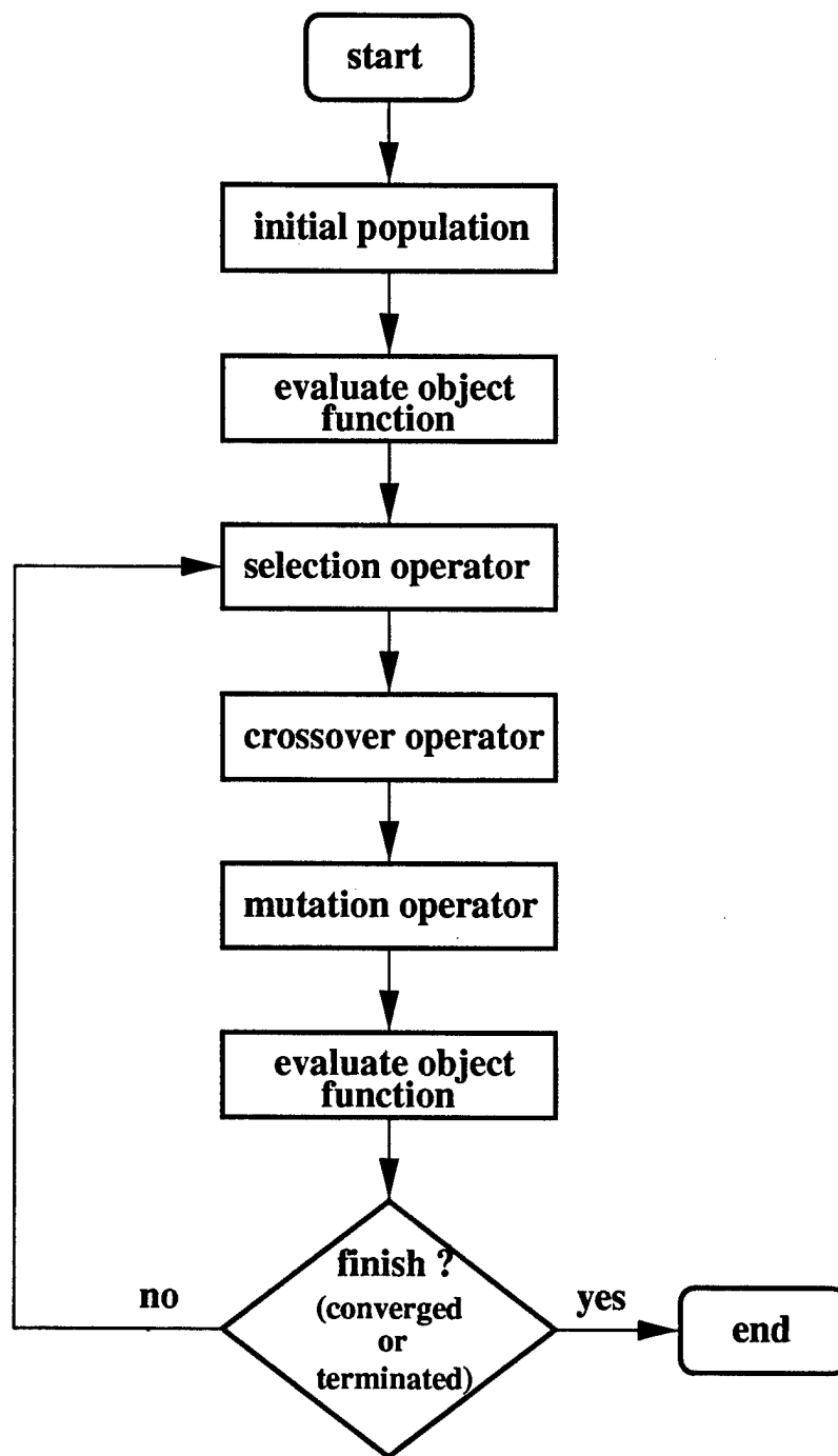
Figure A.1: Flowchart of general genetic algorithm
