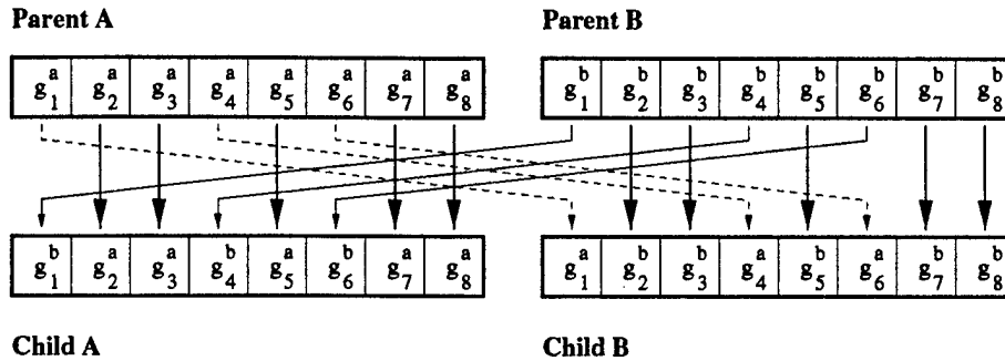
Figure A.7: Uniform crossover operator
