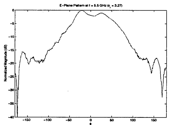
(f) E-Plane pattern at f = 5.5 GHz
