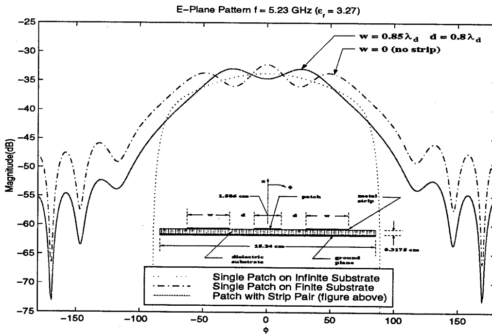
Figure 3.17: Two-strip antenna E-Plane pattern: d=0.8\lambda_d , w=0.85\lambda_d
