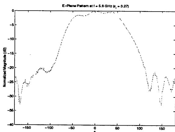
(f) E-Plane pattern at f = 5.8 \text{ GHz}
