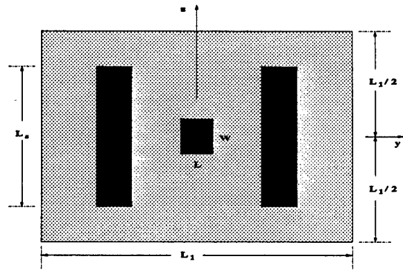
(b) L_s = 6.344 cm
