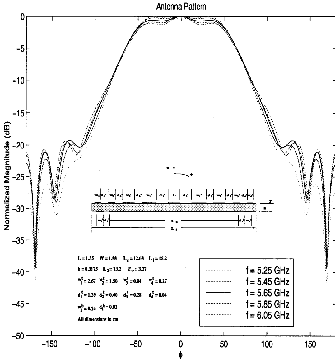
Figure 4.2: Calculated E-Plane pattern of optimized design at different frequencies
