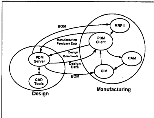
Figure 3. IBP Program Data Flow
