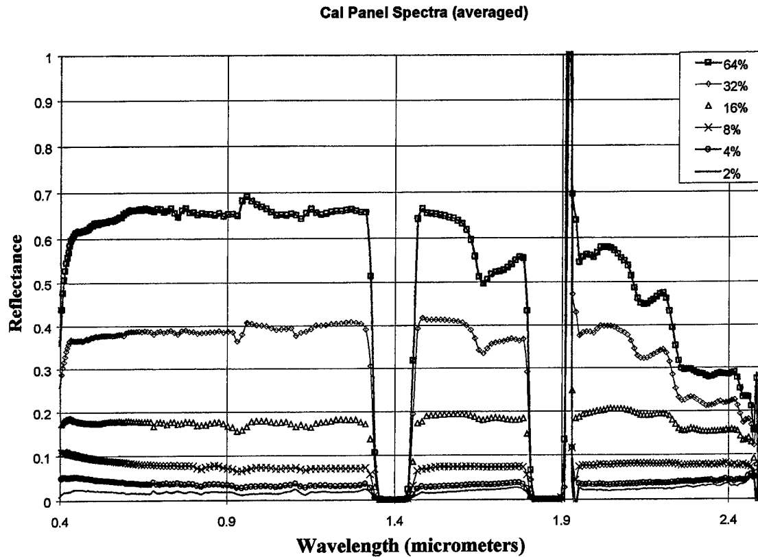
Figure 3.3: Reflectance verses Wavelength for the six step gray scale at Camp Pendleton airfield.
