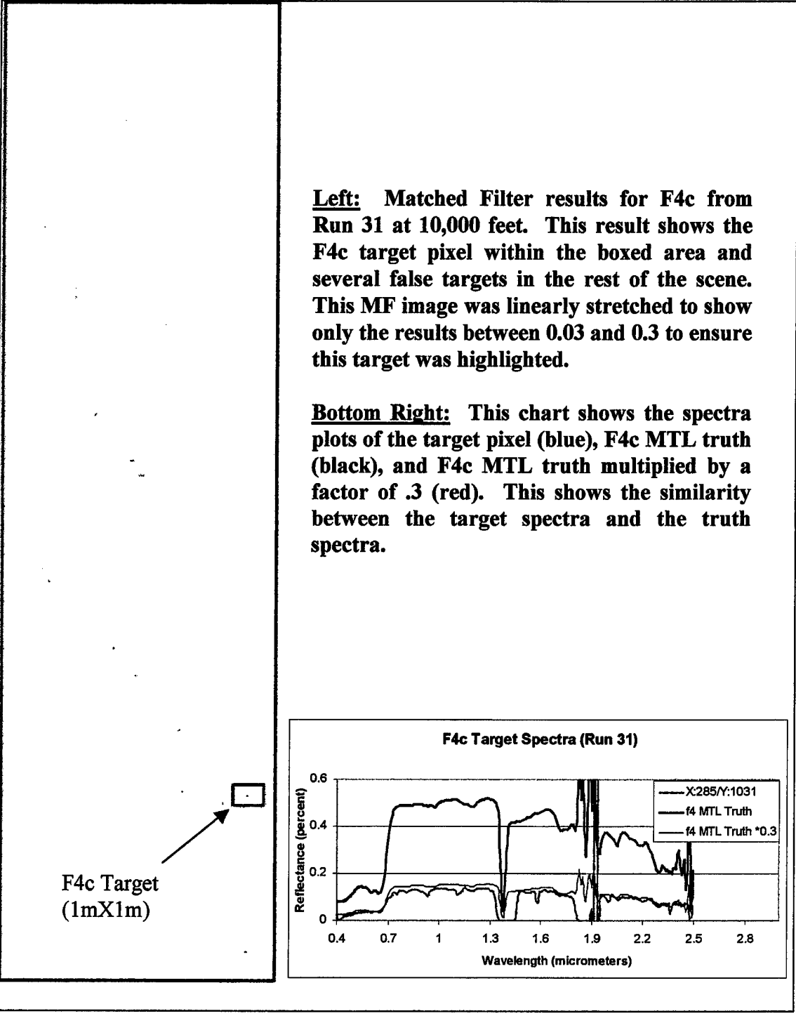
Figure 5.10: Target F4c Matched Filter Detect.
