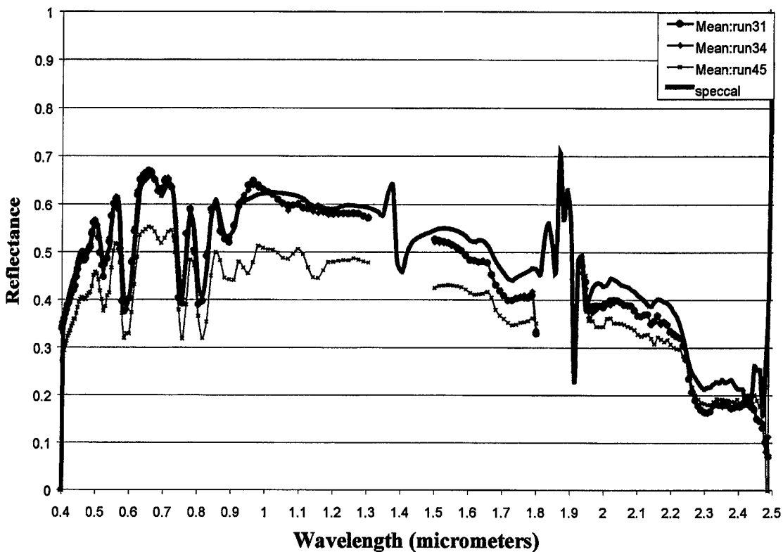
Figure 3.6: Reflectance vs. Wavelength for the Spectral Calibration Panel at Camp Pendleton airfield.
