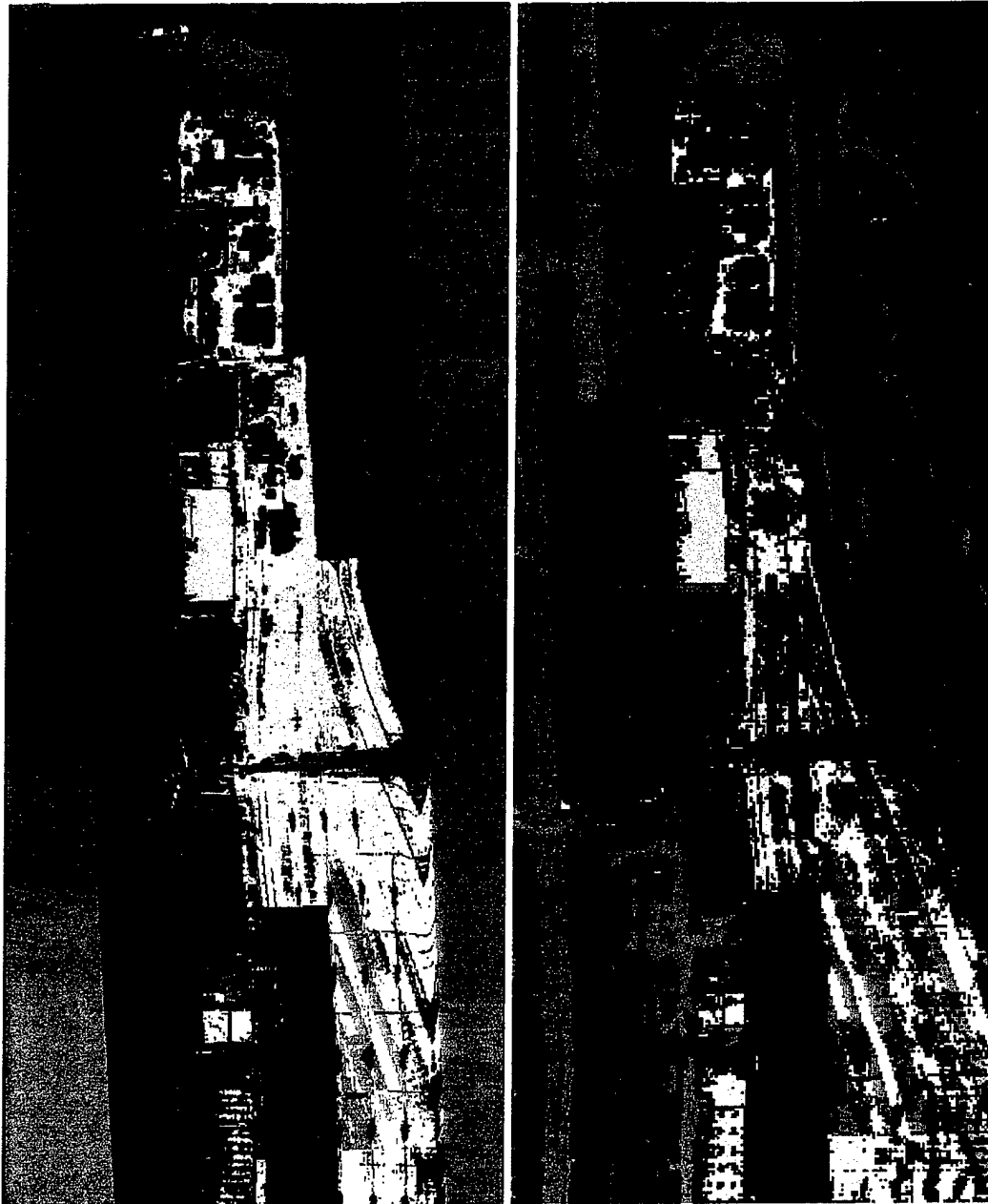
Figure 6: Spectral Angle Mapper results from PC bands 1-10.
