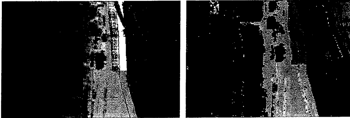
Figure 6.7: Parallelepiped Classification, 5 standard deviations from the mean, results from PC bands 1-10. Left: Run 45 (Warped), samples 0 through 420, lines 450 to 700. Right: Run 31 (X2), samples 0 through 400, lines 300 to 550.
