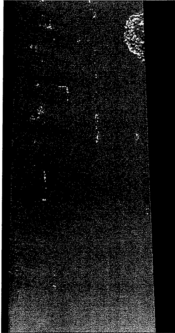
Figure 6.13: Spectral Angle Mapper classification differences between Run 45 (Warped) and Run 31 (X2) from the Camp Pendleton airfield, Littoral Radiance II. White areas represent those classified as vegetation in Run 45, but not in Run 31. Dark gray represents areas classified as vegetation in Run 31, but not in Run 45. The lighter gray represents areas of no difference in classification between the images.
