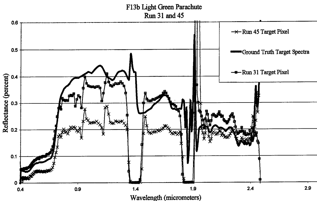
Figure 5.11: Reflectance vs. wavelength for target F13b from Littoral Radiance II, Camp Pendleton airfield Runs 31 (10,000 feet) and 45 (5,000 feet). Note the characteristic reflectance peak for this target in the 1.7 \mu\text{m} wavelength.
