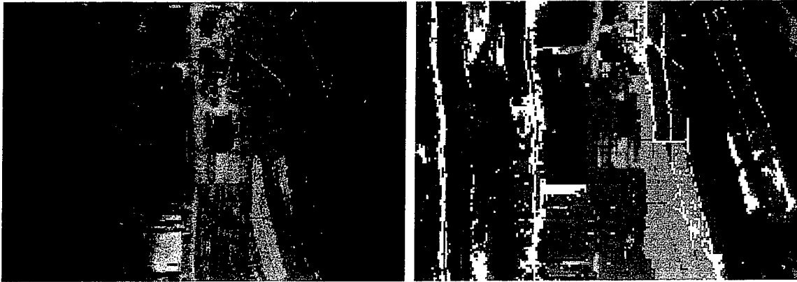
Figure 6.10: Spectral Angle Mapper classification results from the 165 band image cubes. Left: Run 45 (Warped), samples 0 through 420, lines 450 to 700. Right: Run 31 (X2), samples 0 through 400, lines 300 to 550.
