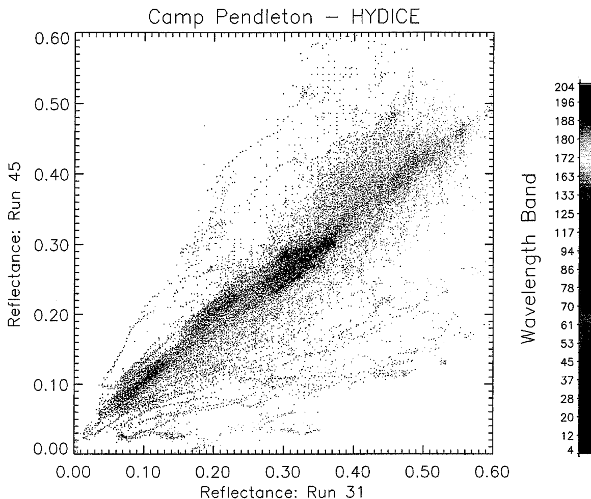
Figure 6.2: Scatter Plot for reflectance data from Run 45 (Warped) and Run 31 (X2). This data was obtained from the Camp Pendleton airfield as part of the Littoral Radiance II Collection in June 1997. The scale on the right shows the representative color for each wavelength band.
