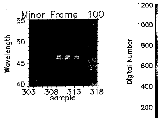
Figure 2.7: Minor Frame 100 from Ivanpah (subset of Figure 2.6 Lamp Position 2). This minor frame shows the wavelength band location (band 46 and 47) of the He/Ne laser.
