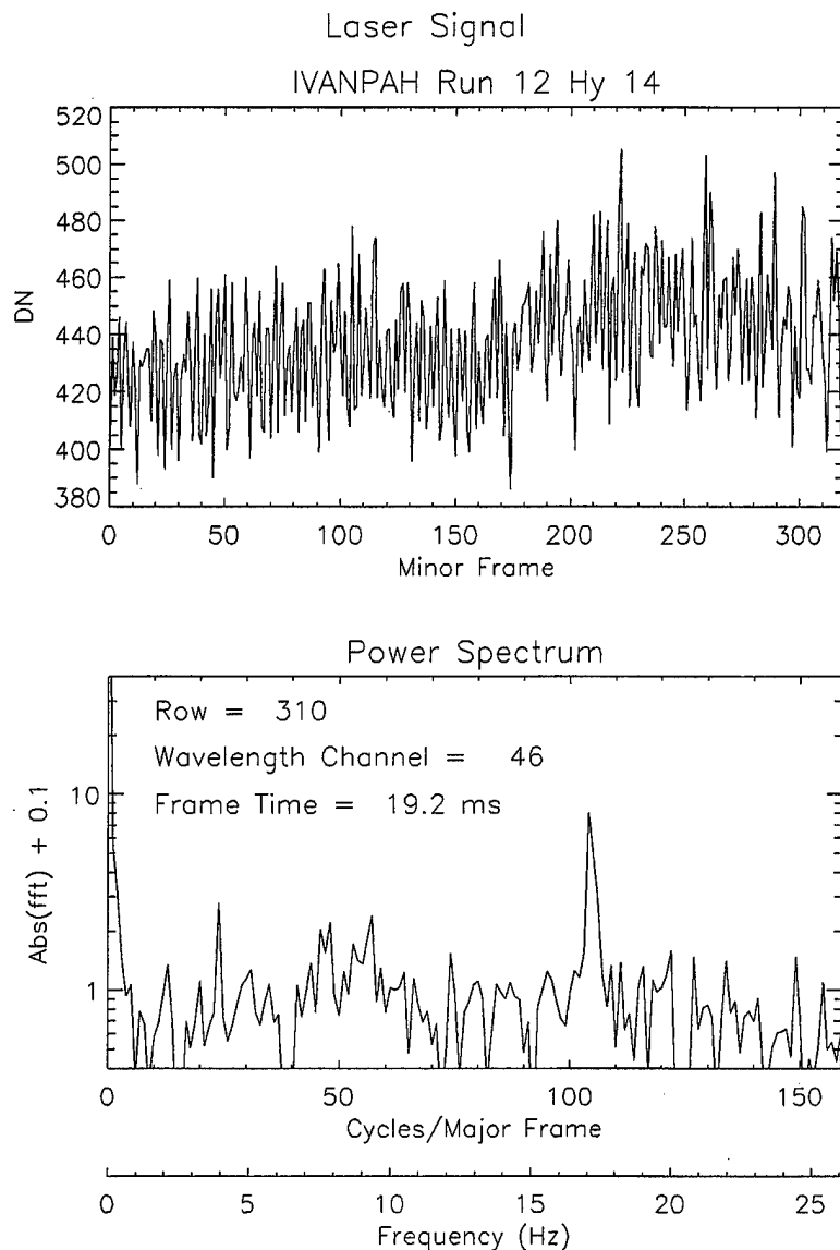
Figure 2.8: He/Ne laser power detected for one wavelength band over 320 minor frames. Top: Resulting DN values from Ivanpah. Bottom: Fast Fourier Transform Power Spectrum.
