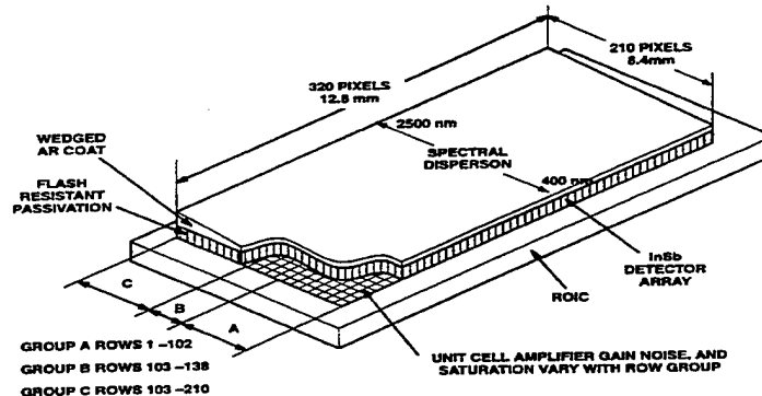
Figure 2.4: Focal plane design. From "HYDICE Focal Plane Design and Performance", (Basedow 1994).
