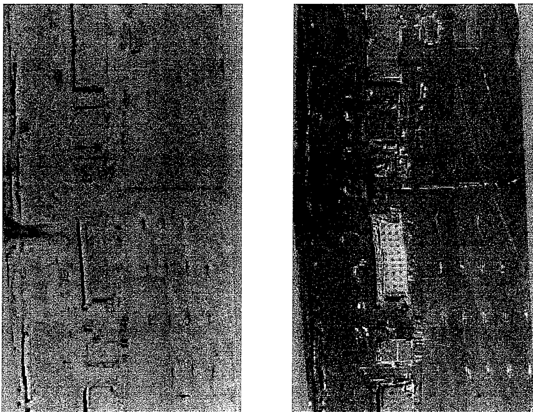
Figure 6.15: Spectral Angle Mapper (SAM) classification differences between Run 45 (Warped) and Run 31 (X2) from the Camp Pendleton airfield, Littoral Radiance II. Left: Bands 6, 7, and 8 from SAM differencing the bands are represented in red, green, and blue respectively. Right: Bands 1, 2, and 3 from SAM differencing the bands are represented in red, green, and blue respectively.
