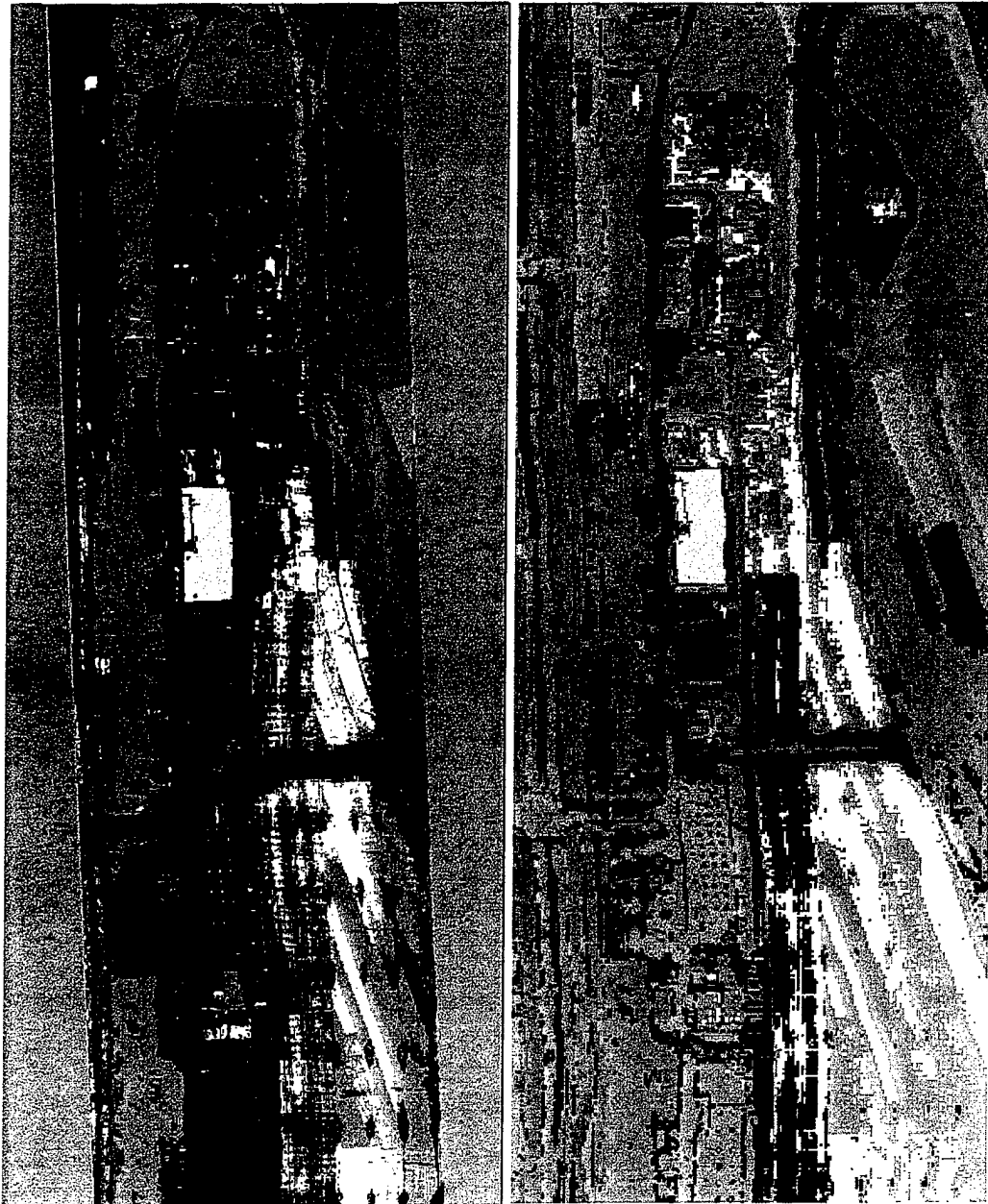
Figure 2: Maximum Likelihood results from PC bands 1-10.
