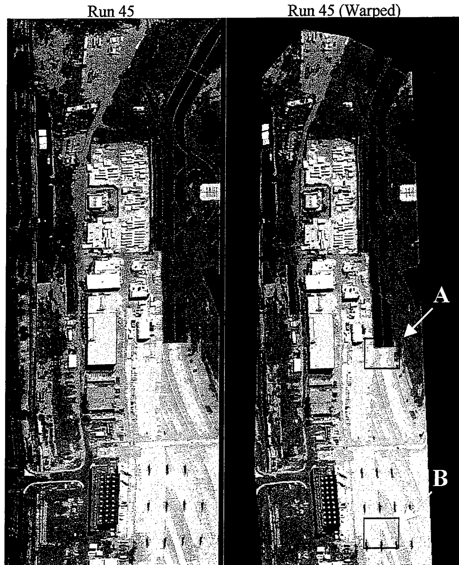
Figure 6.1: Eight-bit palette RGB images (bands 50-40-20) Left: Run 45 (lines 1 to 960) and Right: the resulting Run 45 (Warped) image (lines 1 to 960). The red boxed areas A and B are presented in Figure 6.11.
