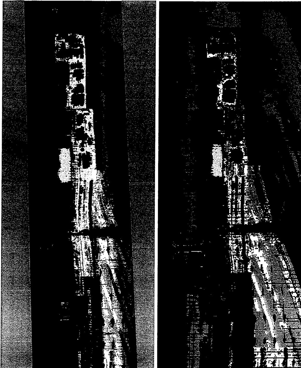
Figure 7: Parallelepiped results from PC bands 1-10, 3 standard deviations from the mean.
