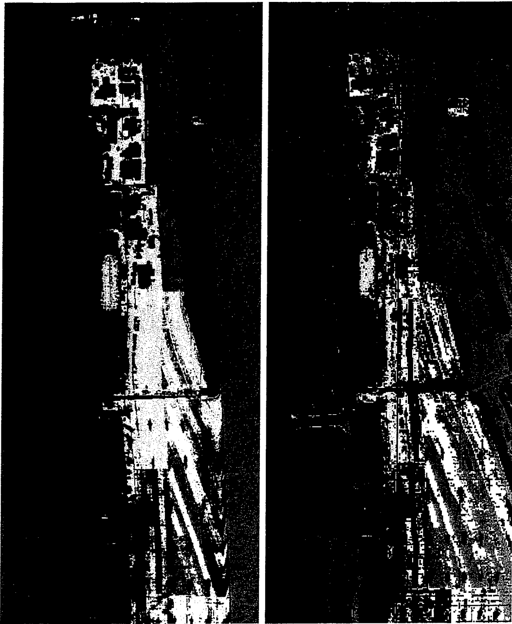
Figure 4: Parallelepiped results from 165 band cube.
