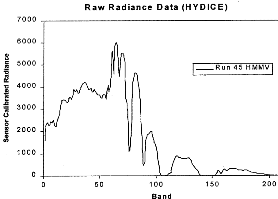
Figure 4.3: HMMV radiance spectra prior to atmosphere removal. This plot represents the pixel spectra of the front hood of a HMMV parked in the scene of Run 45, Camp Pendleton airfield, LR II Experiment.
