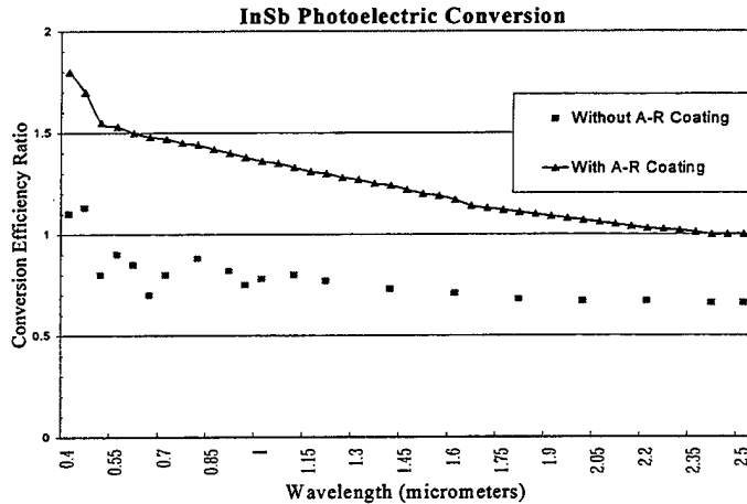
Figure 2.3: Plot of conversion efficiency of InSb versus wavelength (Reproduced figure after Basedow 1992).
