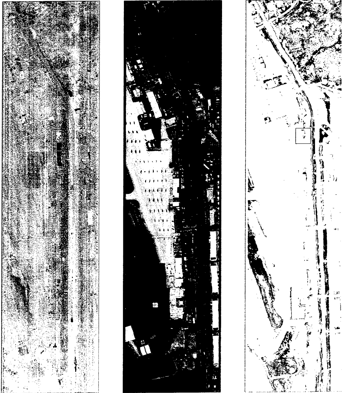
Figure 5.3: The airfield at Camp Pendleton. These are HYDICE images from the Littoral Radiance II experiment, Run 31 at 10,000 feet. Left: Matched Filter result image for target F4a. Right: Spectral Angle Mapper result image for target F4a. A 3 X 3-meter square of Green Nylon, designated F4a, is in the center of the outlined (red box) area.
