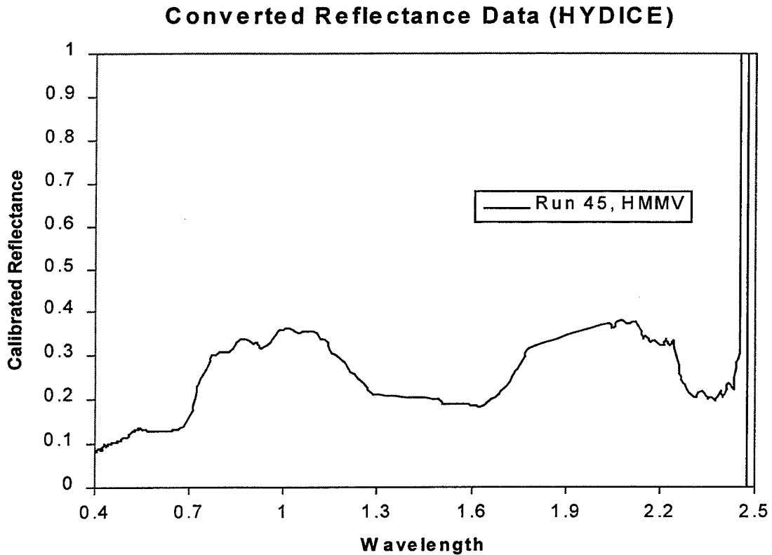
Figure 4.4: HMMV reflectance spectra after ELM calibration. This spectra represents the same pixel as in Figure 4.3 following application of atmosphere correction and normalization.
