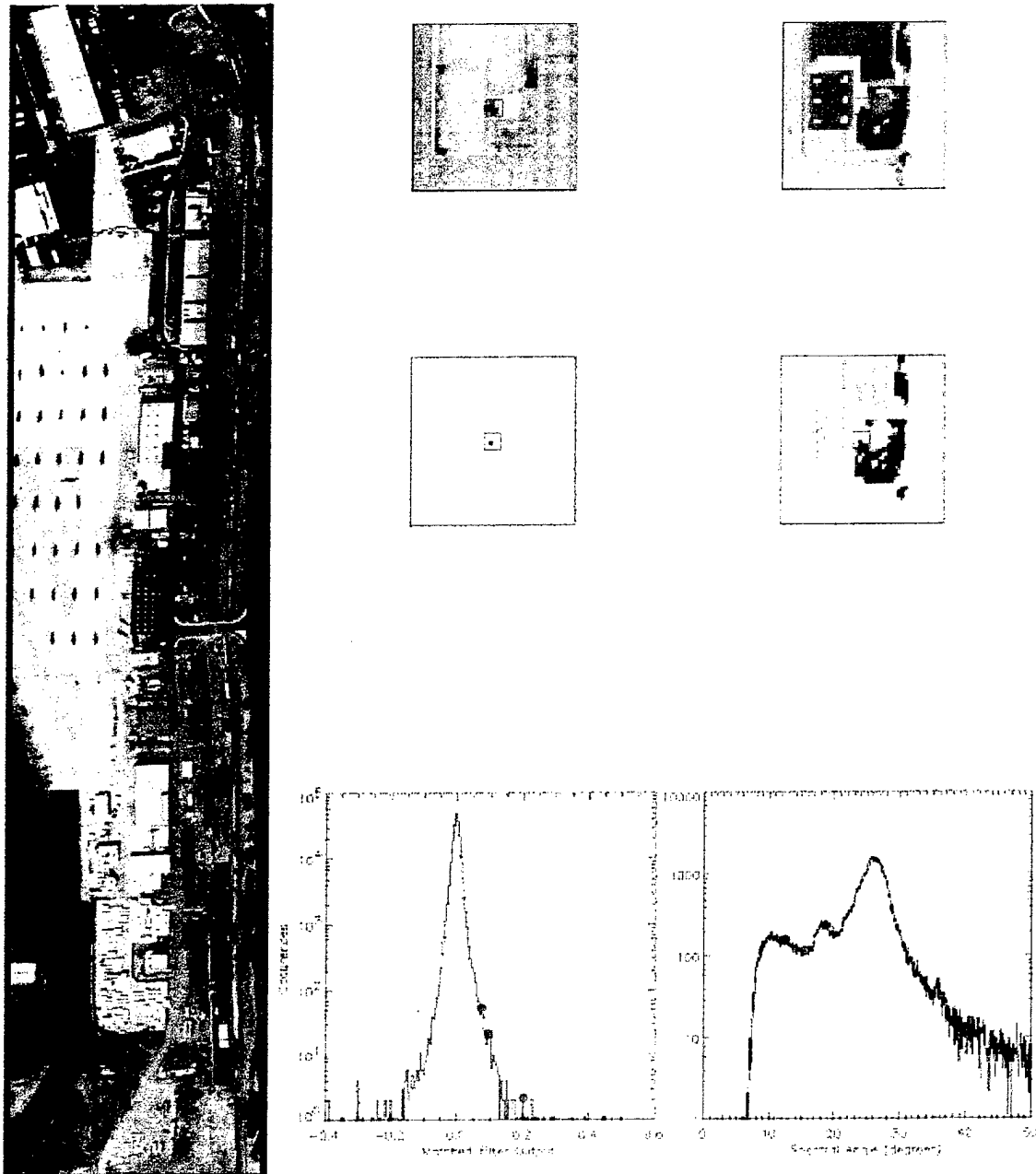
Figure 5.8: Left: HYDICE image of the airfield at Camp Pendleton, Run 45 at 5,000 feet. Top Row: Matched Filter and Spectral Angle Mapper results respectively, for target F4a in the outlined area. Second Row: Result images enhanced to highlight target pixels. Bottom Right: MF and SAM histograms with values for the F4a target pixels marked with red dots. The target pixel values detected by the MF algorithm are greater than three standard deviations from the mean.
