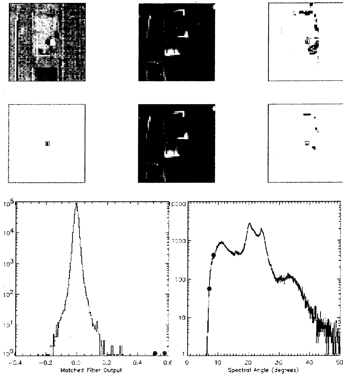
Figure 5.4: The top row contains enlargements of the boxed areas of Figure 5.3. The second row contains the same images enhanced to highlight the target of interest. Left: Matched Filter (MF) result image for target F4a. Center: RGB image of target area. Right: Spectral Angle Mapper (SAM) result image for target F4a. The histograms represent the MF and SAM results respectively, with the target pixels highlighted with red dots. The target pixel values detected by the MF algorithm are greater than ten standard deviations from the mean.
