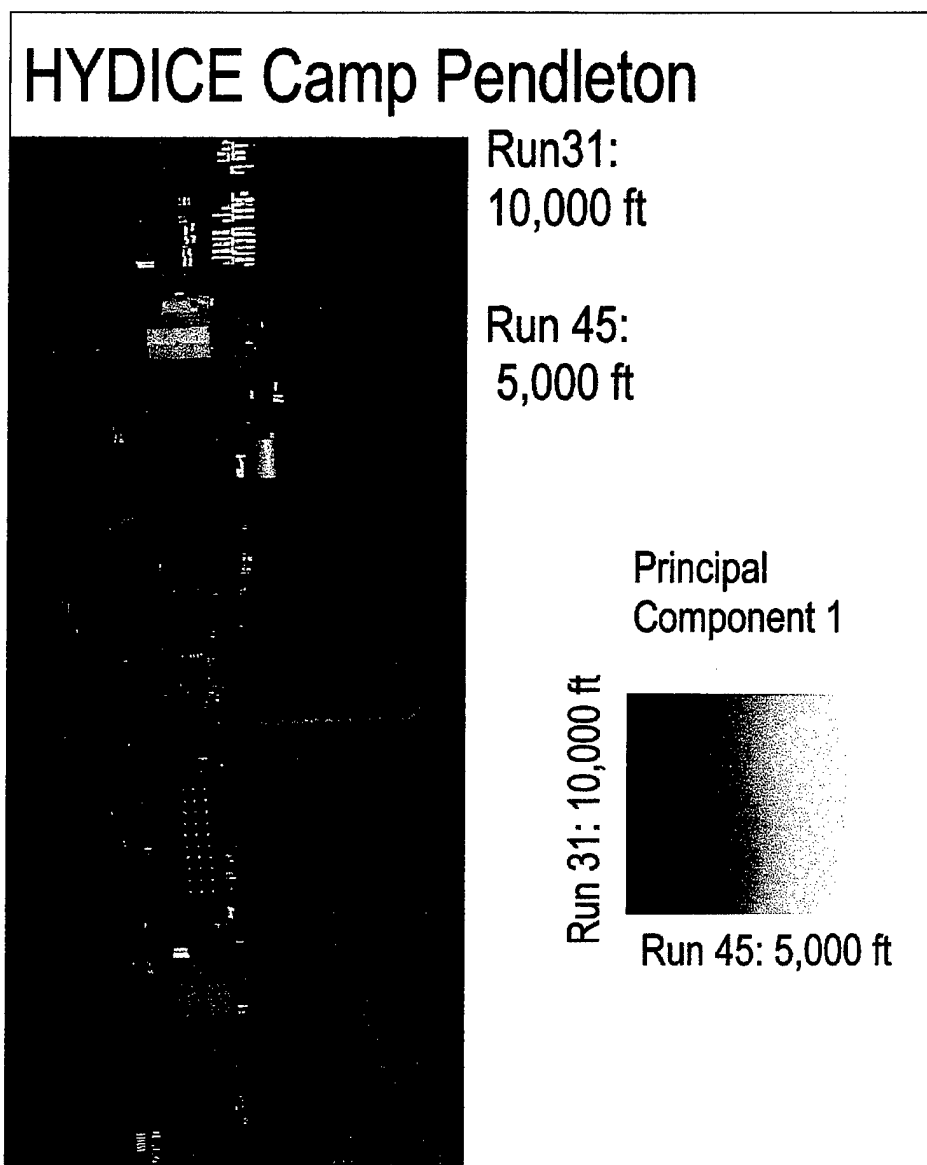
Figure 6.5: Principal Component band 1 (PC1), from Run 45 (Warped) overlaid on PC1-Run 31 (X2). Data obtained from HYDICE flights over Camp Pendleton as part of the Littoral Radiance II collect in June of 1997.
