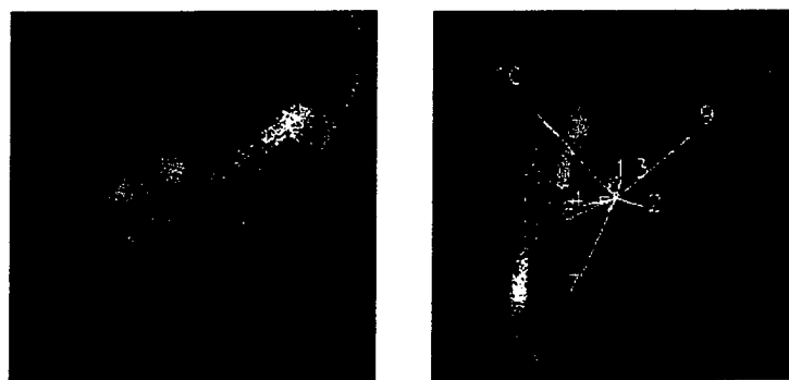
Figure 6.6: Data cloud resulting from the selected regions of interest in Run 45 (Warped) PC bands 1-10. The two pictures show different rotational views of the data cloud with the end members color coded for supervised classifications. The right picture includes the PC axes that resulted from the PC transformations.
