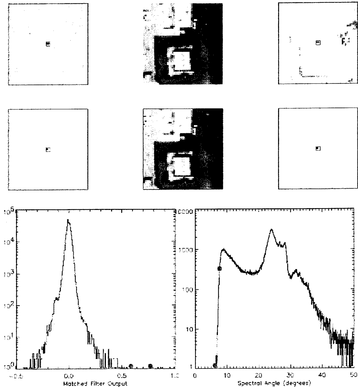
Figure 5.2: The top row contains enlargements of the boxed areas of Figure 5.1. The second row contains the same images enhanced to highlight the target of interest. Left: Matched Filter (MF) result image for target F3a. Center: RGB image of target area. Right: Spectral Angle Mapper (SAM) result image for target F3a. The histograms represent the MF and SAM results respectively, with the target pixels highlighted with red dots. The target pixel values detected by the MF algorithm are greater than ten standard deviations from the mean.
