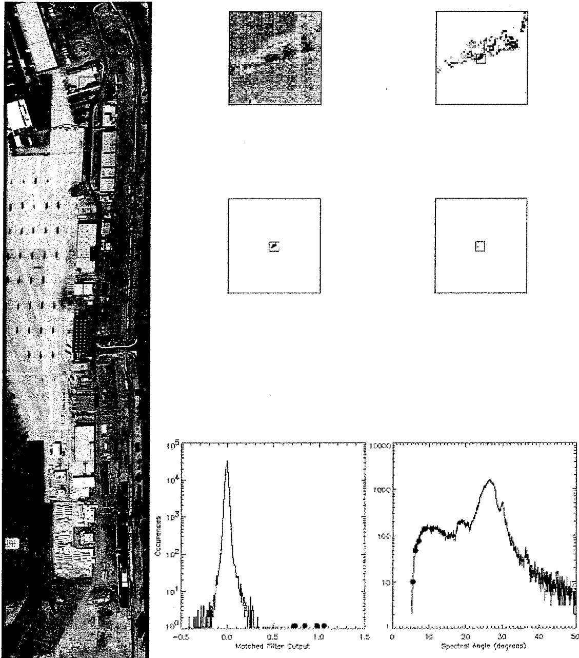
Figure 5.9: Left: HYDICE image of the airfield at Camp Pendleton, Run 45 at 5,000 feet. Top Row: Matched Filter and Spectral Angle Mapper results respectively, for target F12a in the outlined area. Second Row: Result images enhanced to highlight target pixels. Bottom Right: MF and SAM histograms with values for the F12a target pixels marked with red dots. The target pixel values detected by the MF algorithm are greater than ten standard deviations from the mean.
