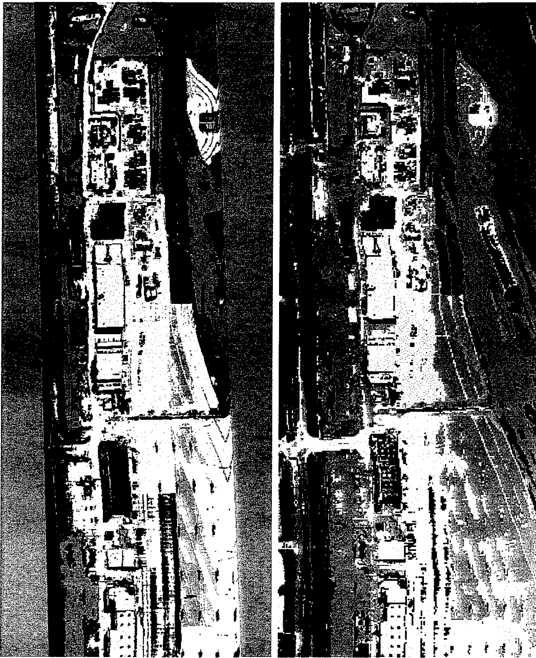
Figure 3: Spectral Angle Mapper results from 165 band cube.
