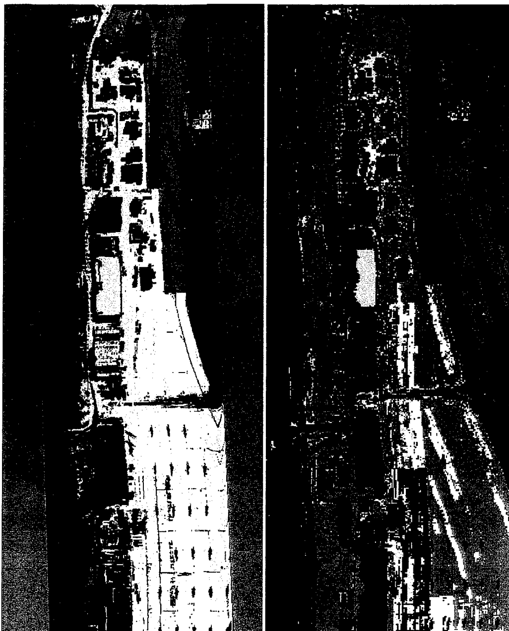
Figure 5: Parallepipiped results from PC bands 1-10 at 5 standard deviations from the mean.
