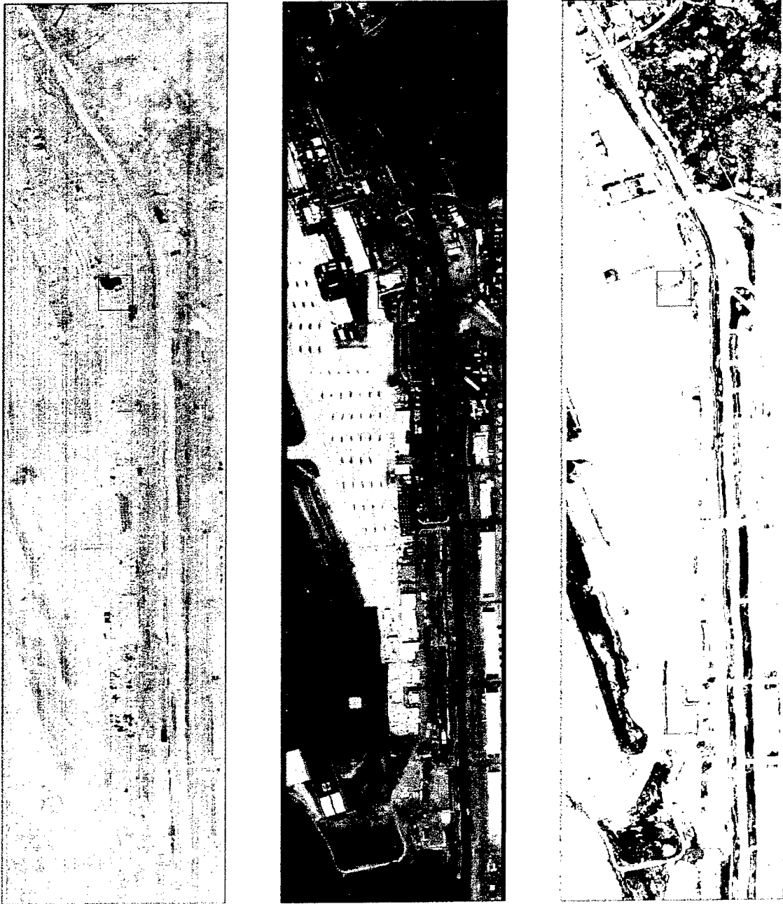
Figure 5.5: The airfield at Camp Pendleton. These are HYDICE images from the Littoral Radiance II experiment, Run 31 at 10,000 feet. Left: Matched Filter result image for target F12a. Right: Spectral Angle Mapper result image for target F12a. A 3 X 3 meter square of Nomex/Kevlar (woodland pattern), designated F12a, is in the center of the outlined (red box) area.
