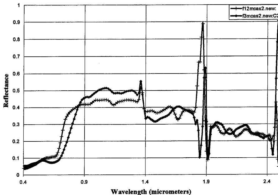
Figure 4.2: MTL Systems, Inc. sampled all target spectra for supplying Ground Truth support for LR II. Spectral plots shown to examine differences between similar green target materials.
