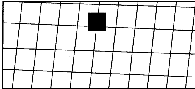
Figure 5.12: Pixel pattern at sensor due to altitude and direction of flight over the target. Although the target area is smaller than the resolved pixel area it still contributes to the reflectance of four separate pixels.
