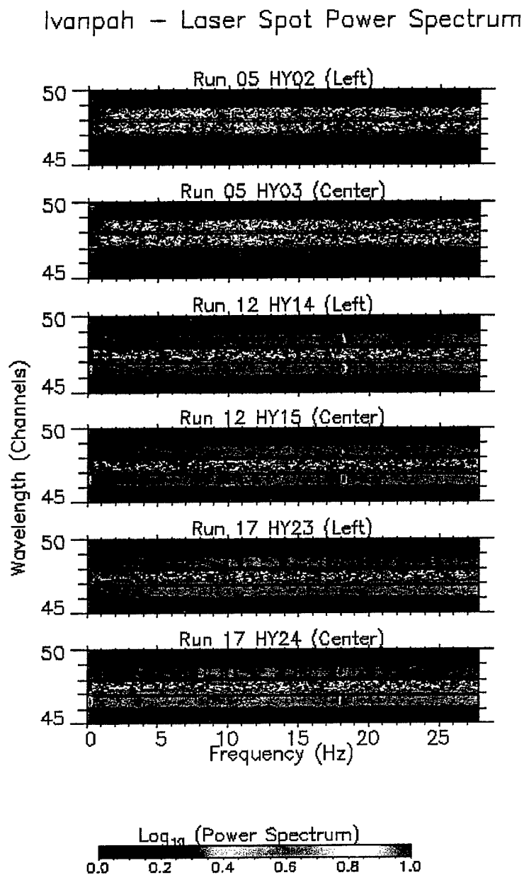
Figure 2.9: Laser Spot Power Spectrum from Ivanpah. This figure shows the Spectral Shift of laser power from bands 47 and 48 in Run 05 to bands 46, 47, and 48 in Run 17.
