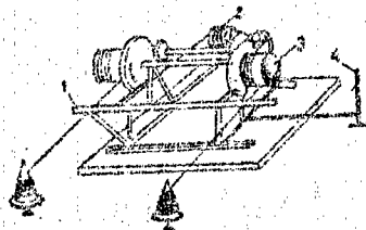
Figure 13 Cold Drawing Machine 1-wire drawing mould; 2-electrically powered machine; 3-winch; 4-switch device
