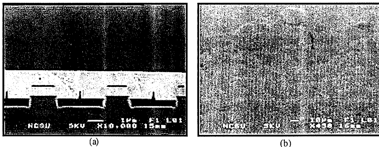
Figure 5. Pendeo-epitaxial growth with coalescence over and between the seed forms resulting in a single GaN layer. 5(a) Cross-section SEM. 5(b) Plane-view SEM.
