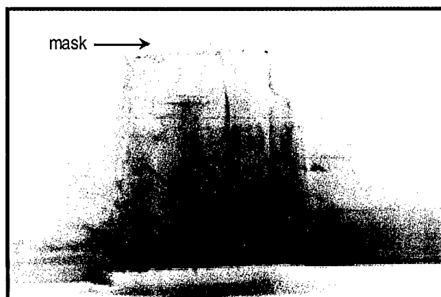
Figure 4. Cross-sectional TEM of a GaN pendeo-epitaxial growth structure showing confinement of threading dislocation under the seed mask, and a drastic reduction of defects in the regrown areas.
