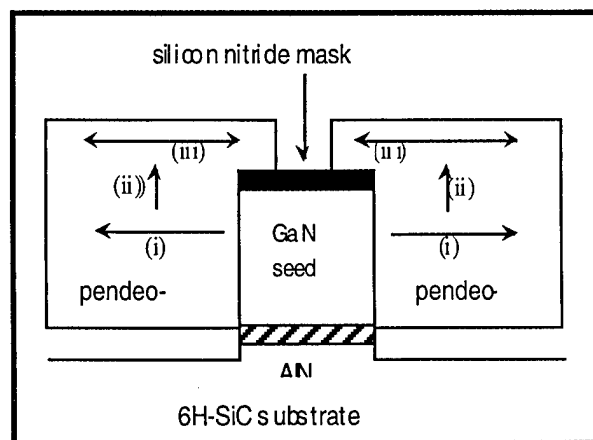
Figure 1. Schematic of GaN pendeo-epitaxial growth process steps.
