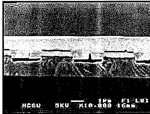
Figure 7. Low magnification cross-sectional SEM of pendeo-epitaxial GaN on a (111)Si substrate and a 3C-SiC transition layer showing coalescence over and between GaN seed forms.
