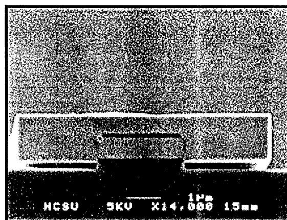
Figure 3. Cross-sectional SEM of a GaN/AlGaN pendeo-epitaxial growth structure showing coalescence over the seed mask.
