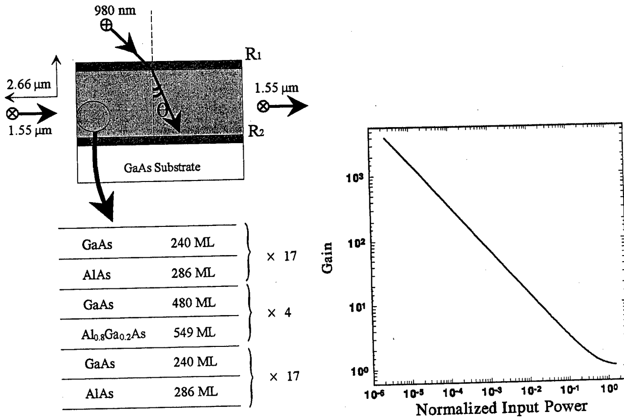
Fig. 1 Left: a new multilayer structure just designed and grown in collaboration with NRL. This device can be used to amplify 1.55 μm and to generate 2.66 μm by mixing 1.55 μm with 980 nm. Right: expected dependence of the gain for the 1.55-μm input beam on the input power normalized by the threshold for oscillation.
