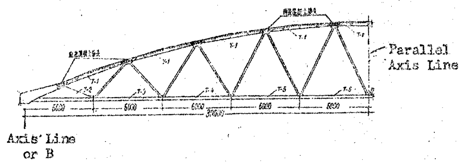
Figure 2 60m Prestressed Concrete Arch-Shape Truss
