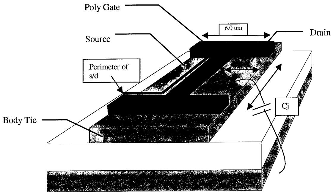
SCHEMATIC REPRESENTATION
