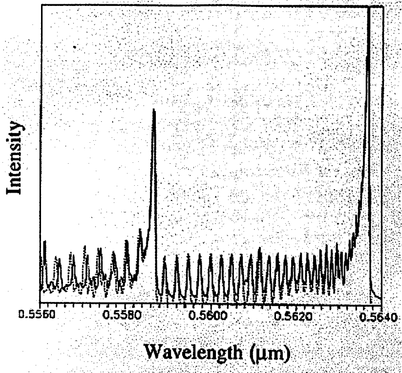
Figure 2.12 An experimental spectrum obtained in a PIA plasma at 100 Torr at Ohio State and fit to a model spectrum (dotted lines). The gas temperature appears to be 1500K.
