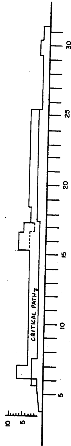
FIG 7-- INSPECTION OF HYDROELECTRIC GENERATING UNIT CLARK HILL PROJECT FINAL TIME-SCALED NETWORK AND MAN-LOADING DIAGRAM.
