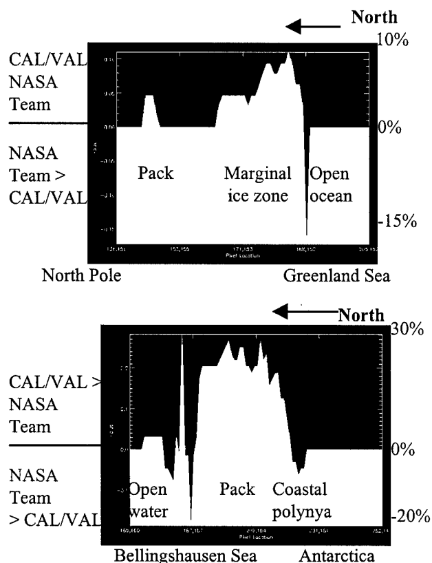
Figure 1. One-dimensional profiles showing CAL/VAL - NASA Team algorithm differences (in % ice concentration) in the Arctic (top figure) and Antarctic (bottom figure).
