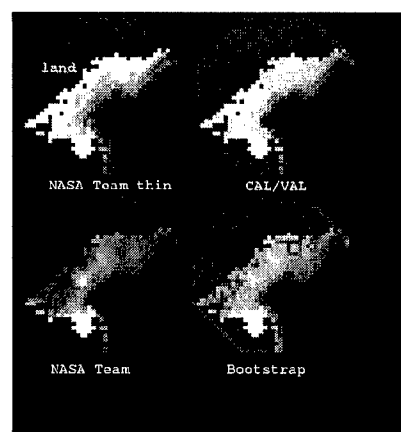
Figure 2. Comparison of algorithms with the NIC ice chart for the Sea of Okhotsk, 9 December 1998. White indicates 100% ice concentration and black 0% ice concentration.
