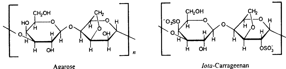
Figure 1. Repeating monomer units of agarose and l -carrageenan, l -car.
