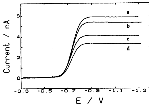
Figure 3. Steady-state voltammograms of reduction of 0.3 mM Tl + in 1% agarose gel (a) without added supporting electrolyte and with (b) 1.5 \times 10^{-5} , (c) 1.5 \times 10^{-4} , and (d) 0.03 M LiClO 4 ; Hg film disk electrode, r = 15 \mu\text{m} , 25 °C.
