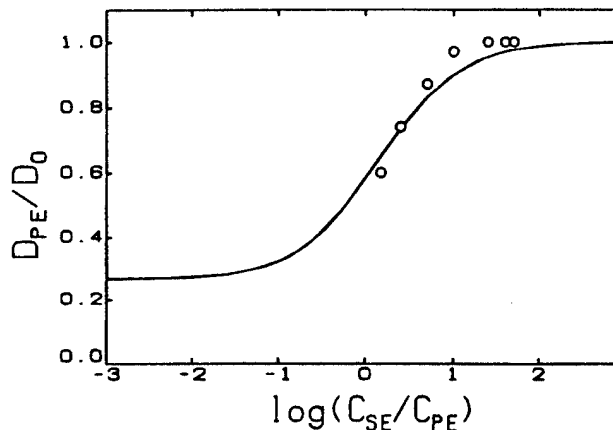
Figure 7. Dependence of the normalized diffusion coefficient of \text{Tl}^+ probe (O) in 0.5% \iota -car gel, D_{PE}/D_0 , on the concentration of electrolyte, \text{LiClO}_4 , \log(C_{SE}/C_{PE}) . (—) calculated according to the Manning's theory, with b = 0.22 nm.
