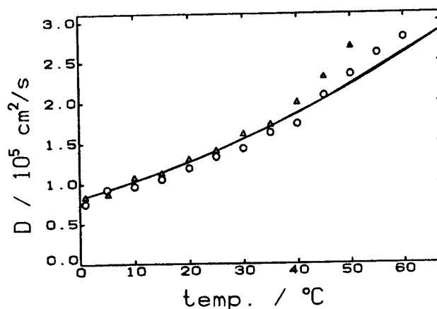
Figure 5. Dependence of the diffusion coefficient of Tl^+ on temperature: (O) 0.3 mM Tl^+ in 0.5% l -car gel with 1 M LiClO_4 ; ( \Delta ) 0.3 mM Tl^+ in 1 M LiClO_4 solution; (—) calculated from eq 3 and the experimental diffusion coefficient at 25 °C for Tl^+ in 1 M LiClO_4 solution.
