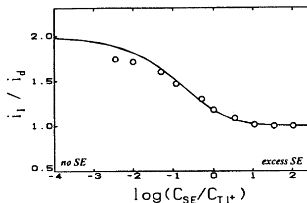
Figure 4. Dependence of normalized limiting currents (wave height in the presence of excess supporting electrolyte = 1) on concentration of supporting electrolyte (SE), LiClO 4 , for 0.3 mM Tl + reduction in 1% agarose gel. (—) theoretical plot for +1-1 substrate in univalent electrolyte, eq 2. 43
