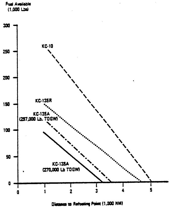
FIGURE IV-3 TANKER COMPARISON (Radius Mission)
