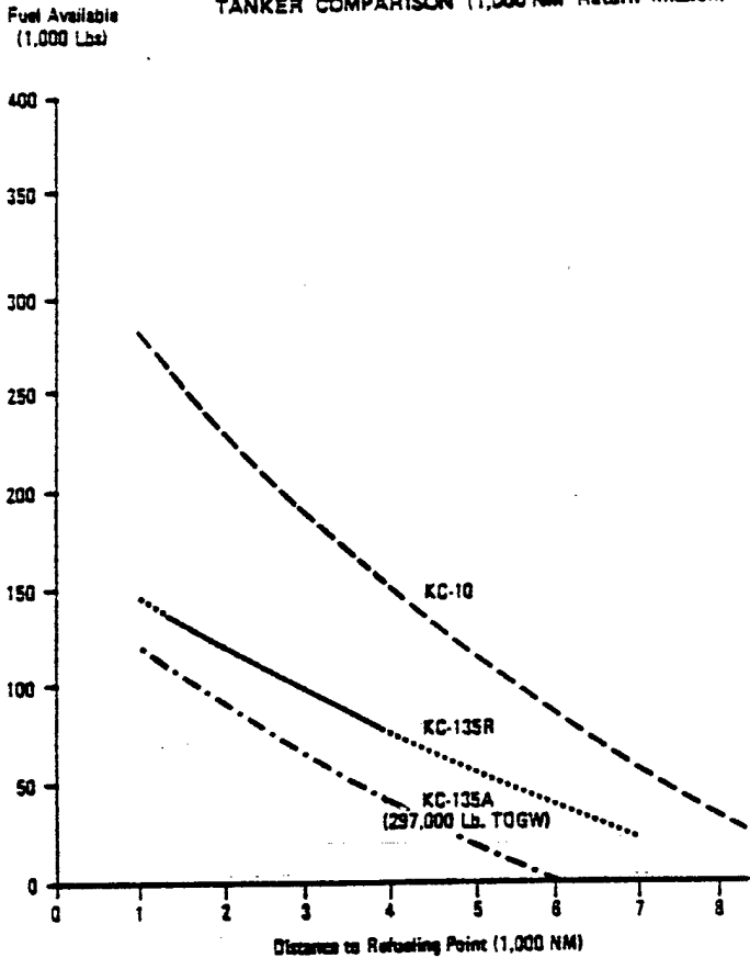
FIGURE IV-2 TANKER COMPARISON (1,000 NM Return Mission)
