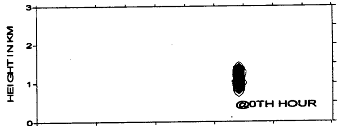
Fig. 4 Empirical cloud profile at the zeroth hour
