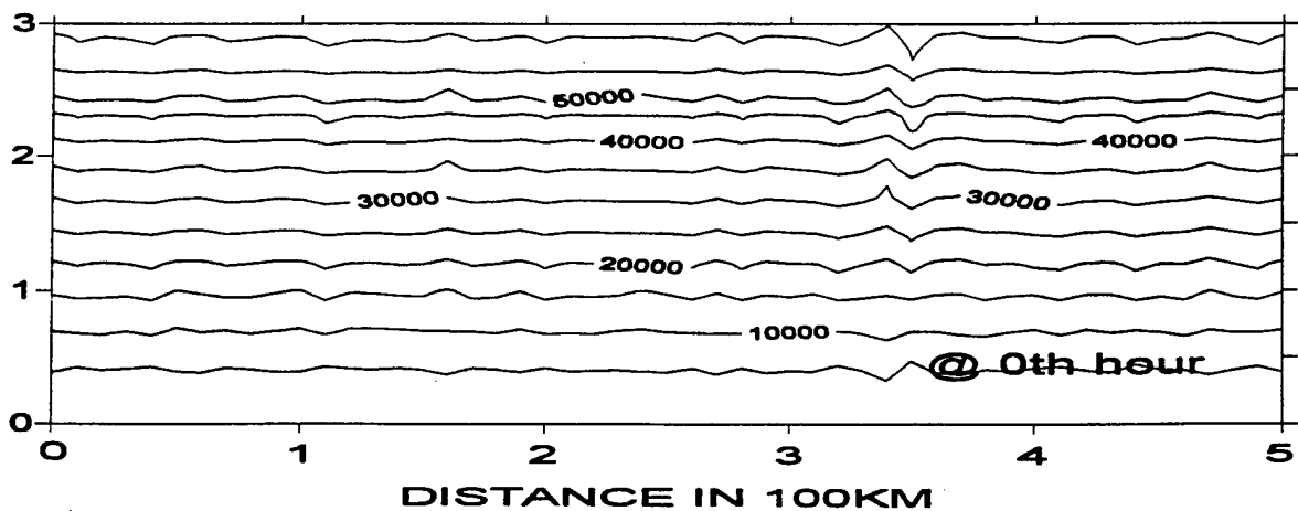
Fig. 8: Contours of a set of retrieved experimental stream function values
