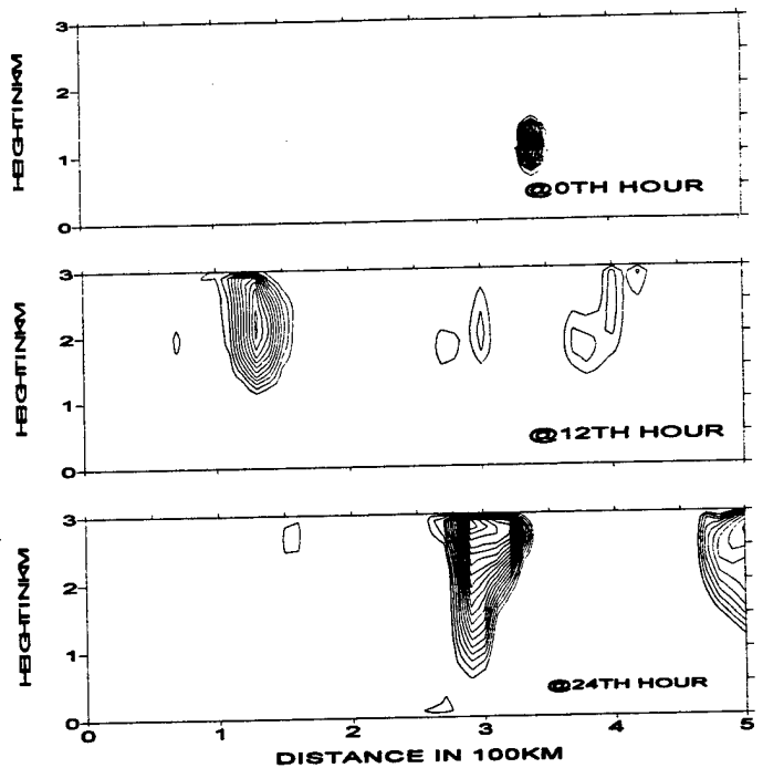
Fig. 5 Snapshots of predicted cloud profiles
