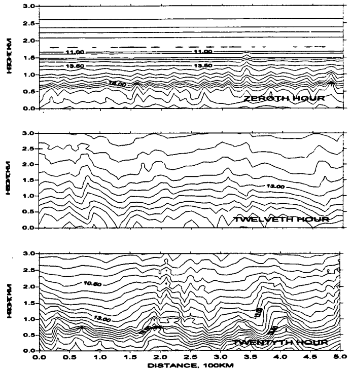
Fig. 2 Contours of empirical total moisture mixing ratio
