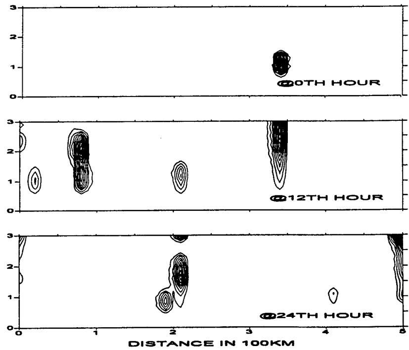
Fig. 11: Contours of experimental total moisture mixing ratio
