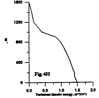
Fig. 4: Predicted Mean Quantities and Turbulent Fluxes 4A - Mean velocity; 4B - Reynolds stress; 4C - Potential temperature; 4D - Thermal flux; 4E - Total moisture ratio; 4F - Moisture flux; 4G - Liquid moisture ratio; 4H - Turbulent energy.
