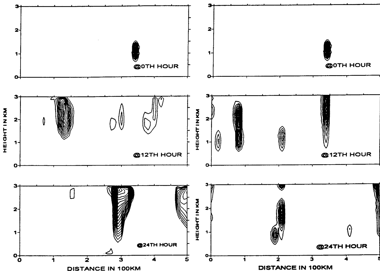
Fig. 14B: Empirical Cloud Profiles
