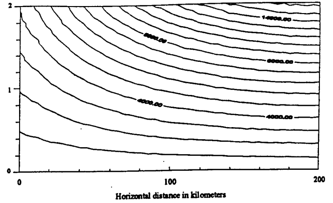
Fig. 3: Contours of Superposed Stream Functions with Entrainment at the Top
