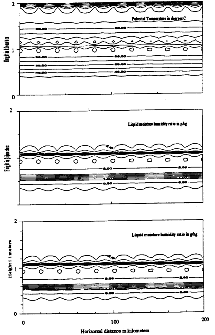
Fig. 4: Initial Steady state at the Zeroth Hour
