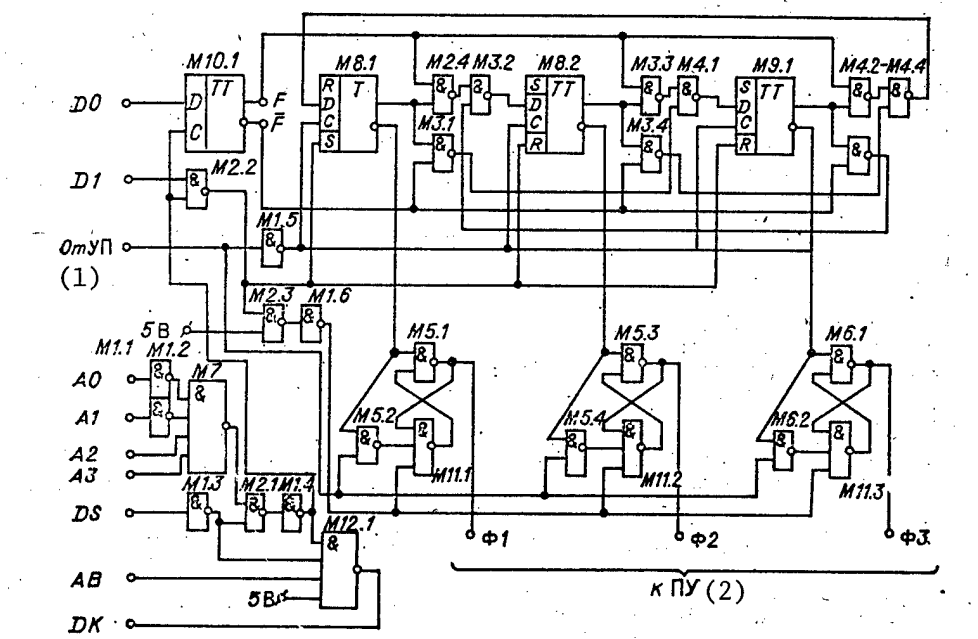
Figure 3. Diagram of Signal Phase Shaper: M1--K155LN1; M2-M6--K155LA3; M7--K155LA2; M8 and M9--K155TM2; M10--K155TM7; M11--K155LA4; M12--K155LA7
