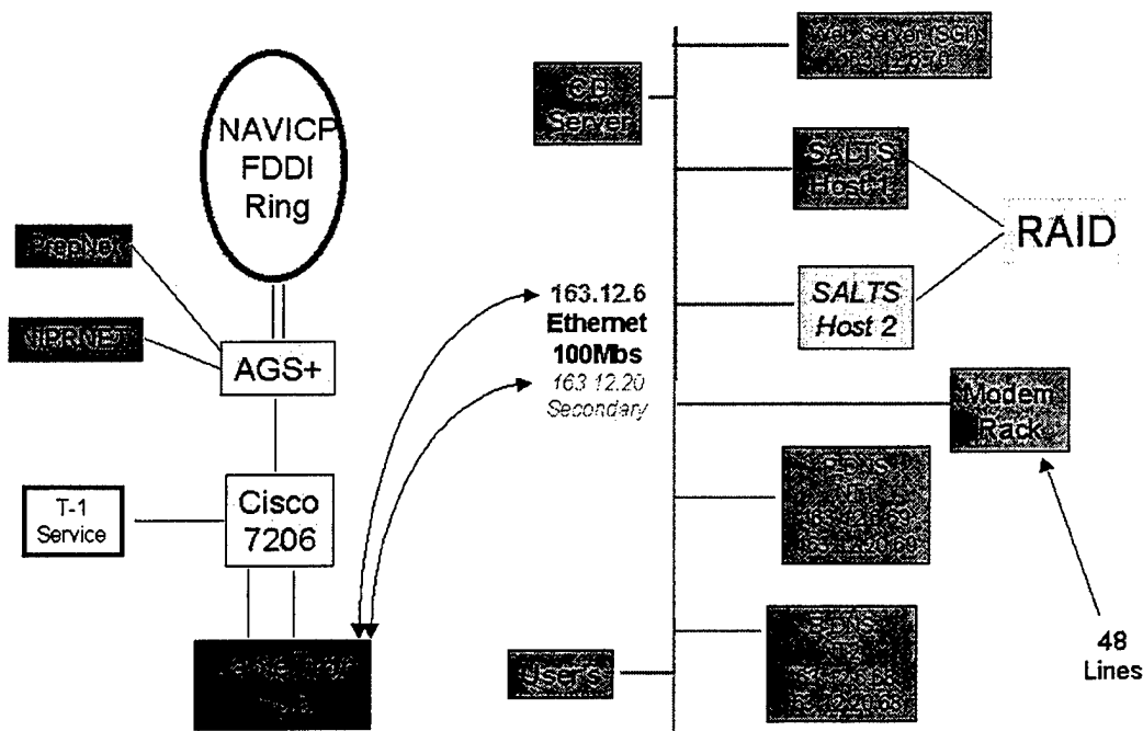
Figure 6 SALTS Hardware Upgrade
