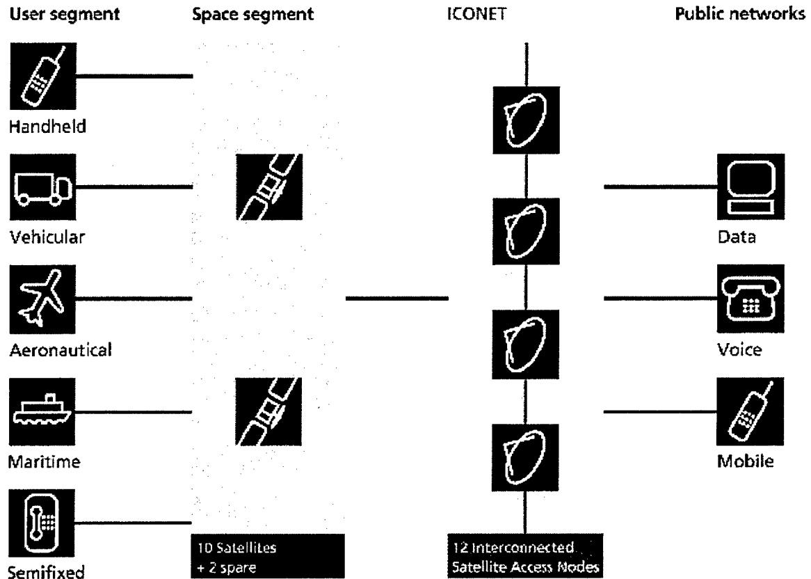
Figure 12 ICO System From Ref. [17]
