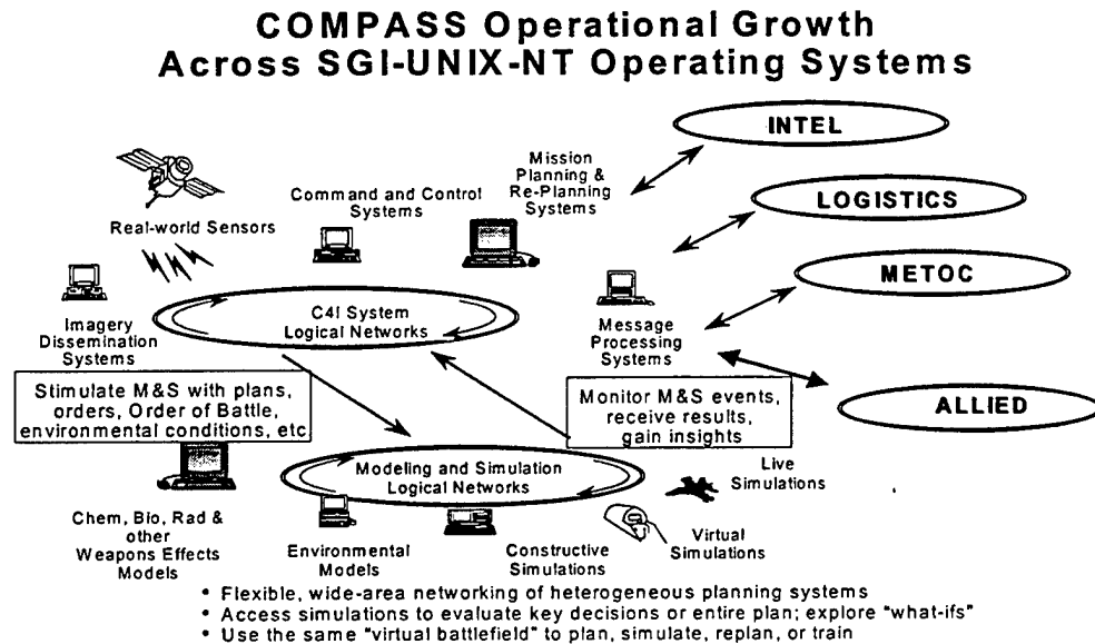
Figure 2. 2 SPAWAR Presentation Slide of COMPASS. After Ref.[MCSW99]
