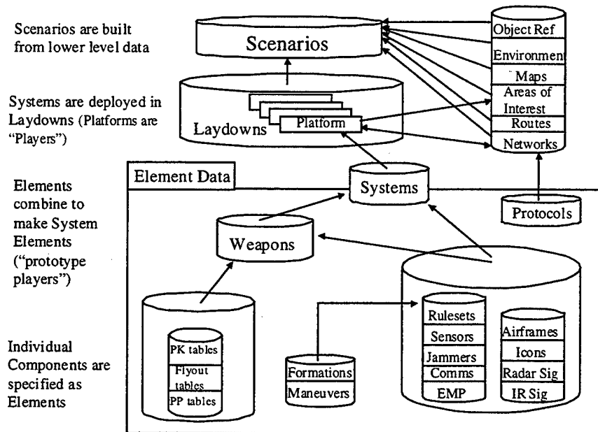
Figure 3. 4 Hierarchy of Data Builds an EADSIM Scenario. After Ref. [TELE98]
