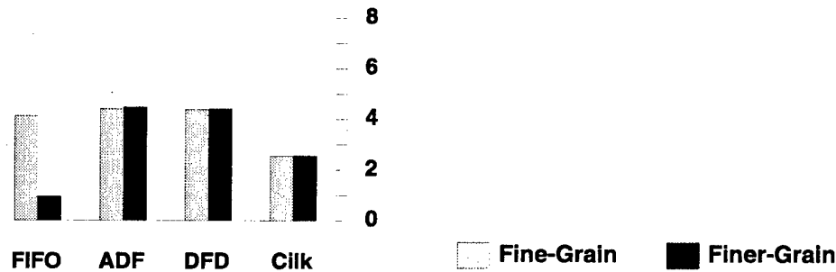
Figure 7.6: Speedups for the octree-building phase of Barnes Hut (for 1M particles). The phase involves extensive use of locks on cells of the tree to ensure mutual exclusion. The Pthreads-based schedulers (all except Cilk) support blocking locks.
