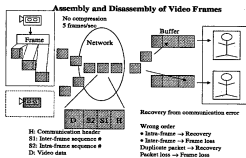
Figure 15: The Assembly and Dis-assembly of Video Frames.
