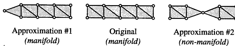
Figure 2.2: Two approximations of the same surface, both constructed by contracting a single edge.
