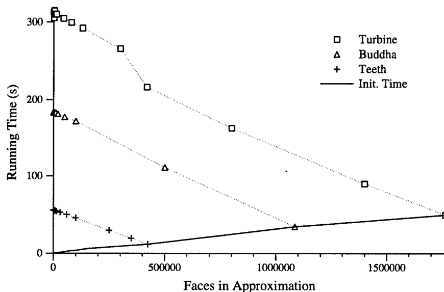
Figure 6.4: Running times for large-size models ( n > 400,000 faces).
