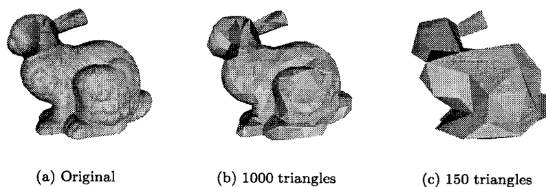
Figure 9.1: Sample approximations of a scanned bunny surface model containing 70,000 triangular faces.
