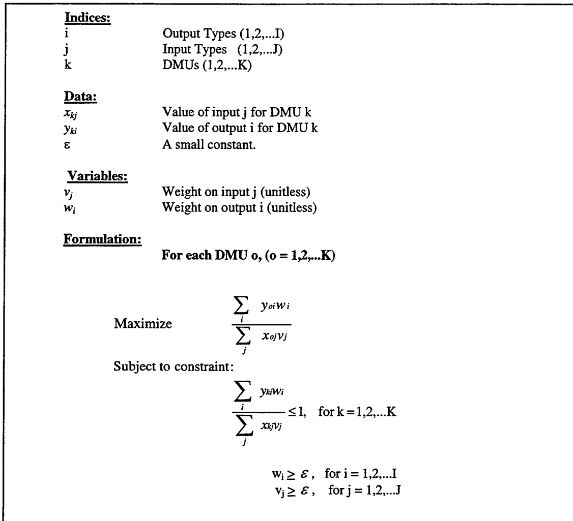
Figure 1. CCR DEA Model Formulation (Norman, 1991, p. 235)
