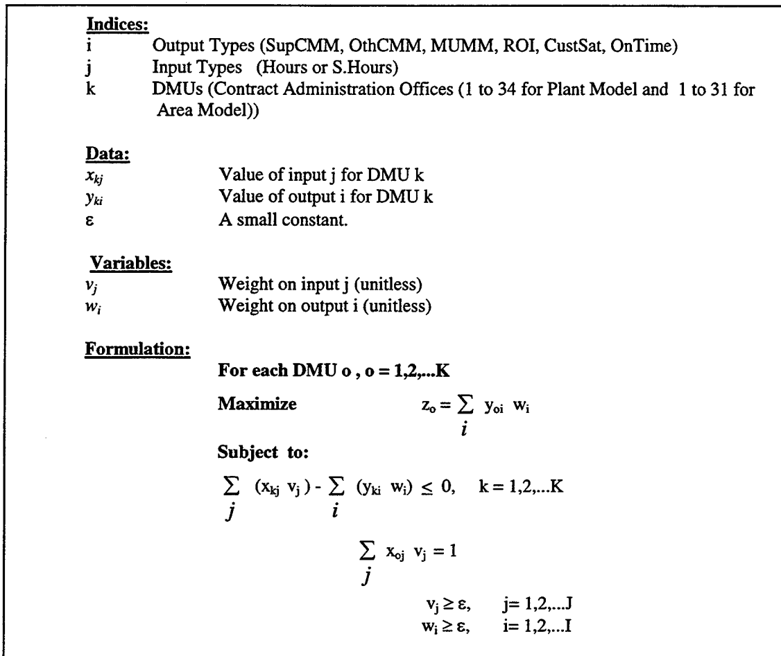
Figure 5. Linearized CCR Formulation (Norman, 1991, p. 236)
