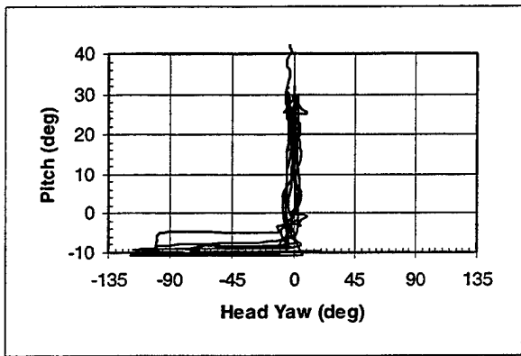
Aircraft Pitch vs. Head Yaw (AF - 10-60)
