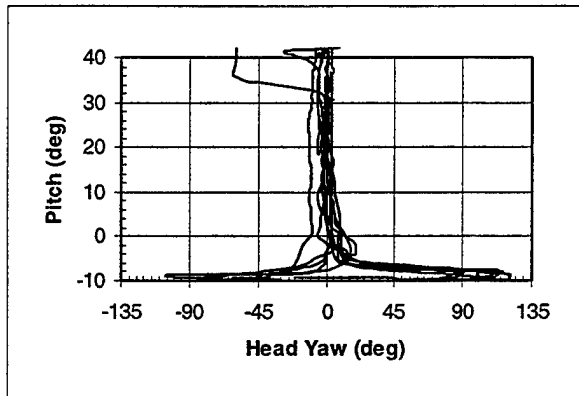
Aircraft Pitch vs. Head Yaw (A - 10-30)
