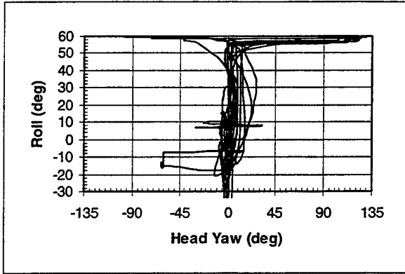
Aircraft Roll vs. Head Yaw (A - 20-60)
