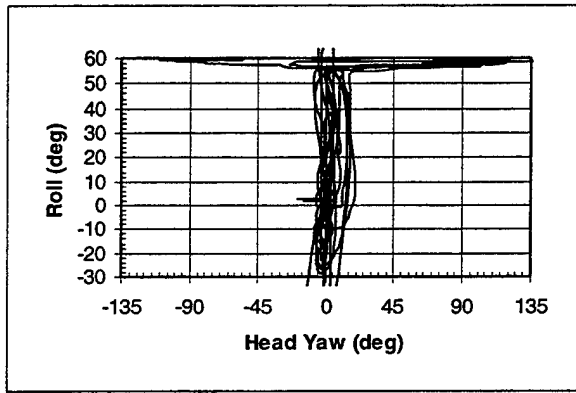
Aircraft Roll vs. Head Yaw (AF - 20-60)
