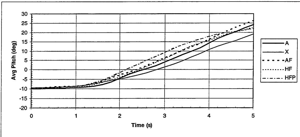
Average Pitch History Comparison (10-60)
