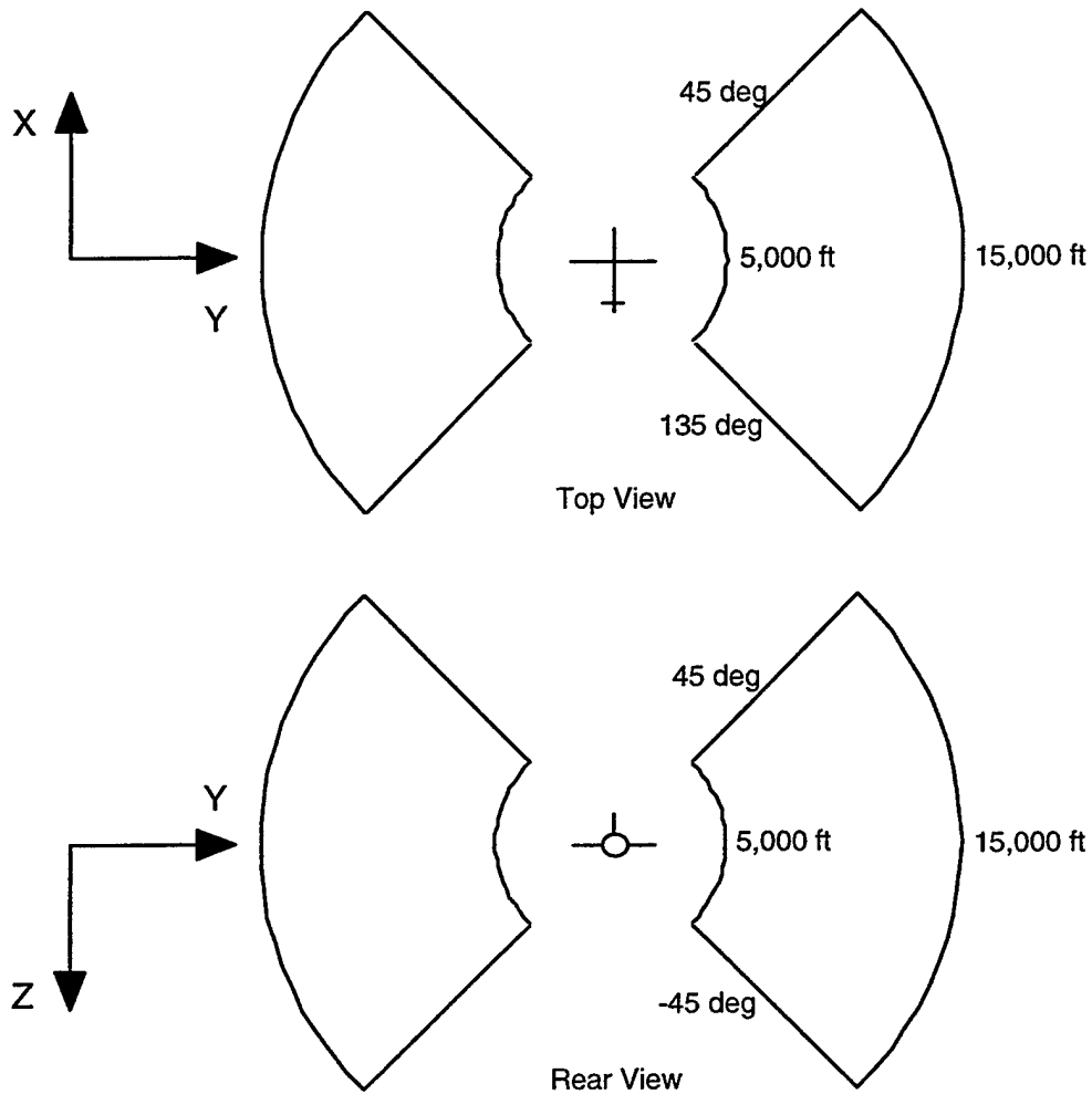
Figure 3.6 Target Boundaries
