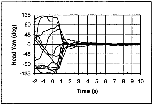
Head Yaw Histories (AF - 20-30)
