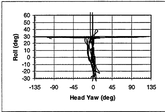
Aircraft Roll vs. Head Yaw (AF - 20-30)
