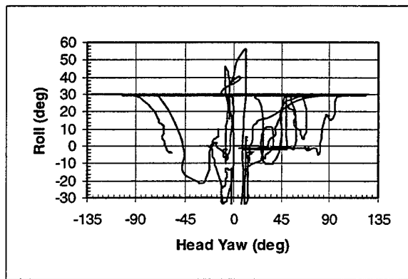
Aircraft Roll vs. Head Yaw (HFP - 10-30)
