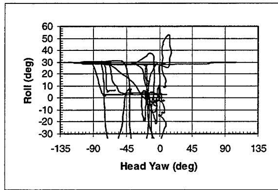
Aircraft Roll vs. Head Yaw (HFP - 20-30)
