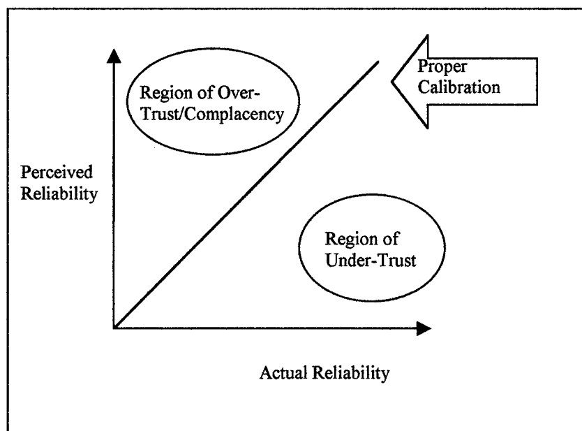
Figure 2: Reliability calibration
