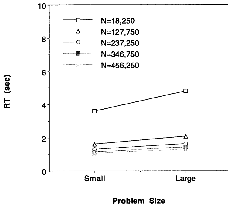
Figure 3.1: The Effect of Problem Size across Grades: (a) Data; (b) Model.
