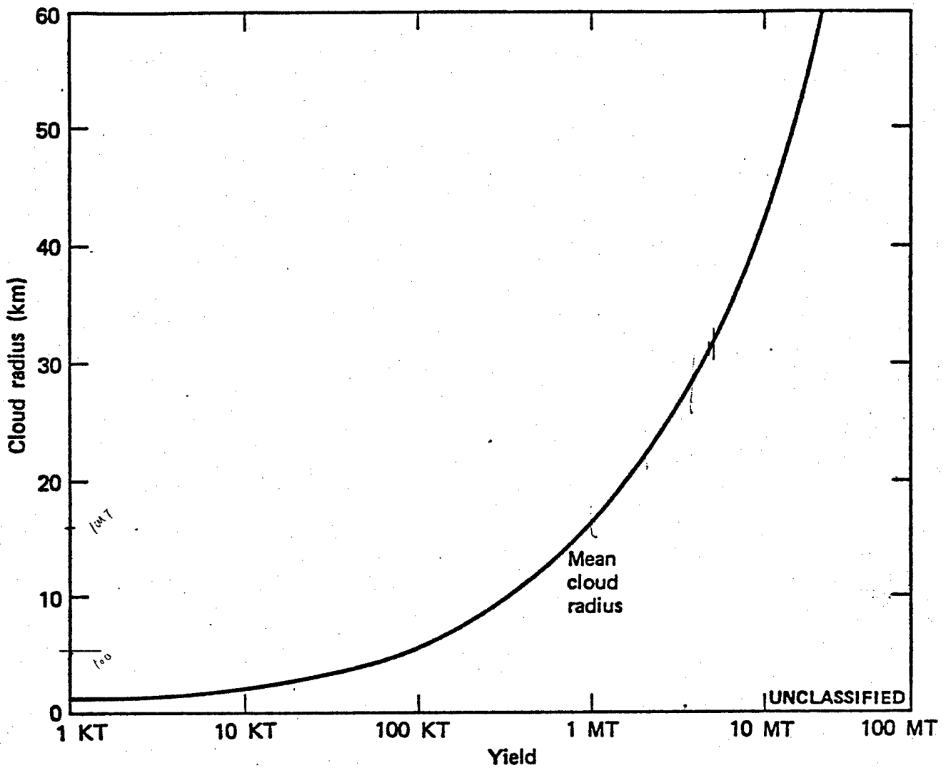
(U) Low-altitude burst cloud mean radius vs yield at stabilization time. 10^3 \text{ sec}
