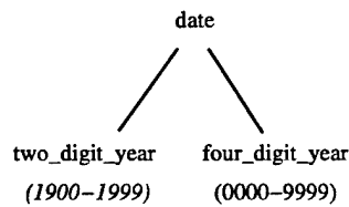
Figure 15: A Second Y2K Interpretation: A converter K_2 : \text{two\_digit\_year} \rightarrow \text{four\_digit\_year} respects date , where K_2 adds 1900 to the two\_digit\_year value.
