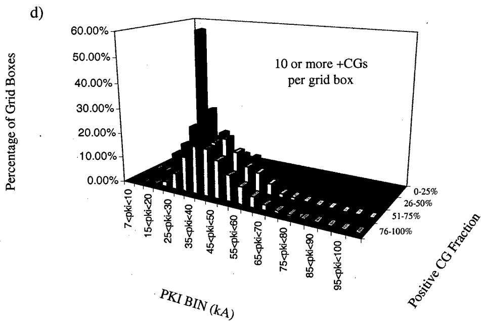
Figure 4.7: Normalized three-dimensional frequency distributions of average positive peak current as a function of positive CG fraction for grid boxes containing (c) four or more positive CGs per grid box and (d) ten or more positive CGs per grid box.
