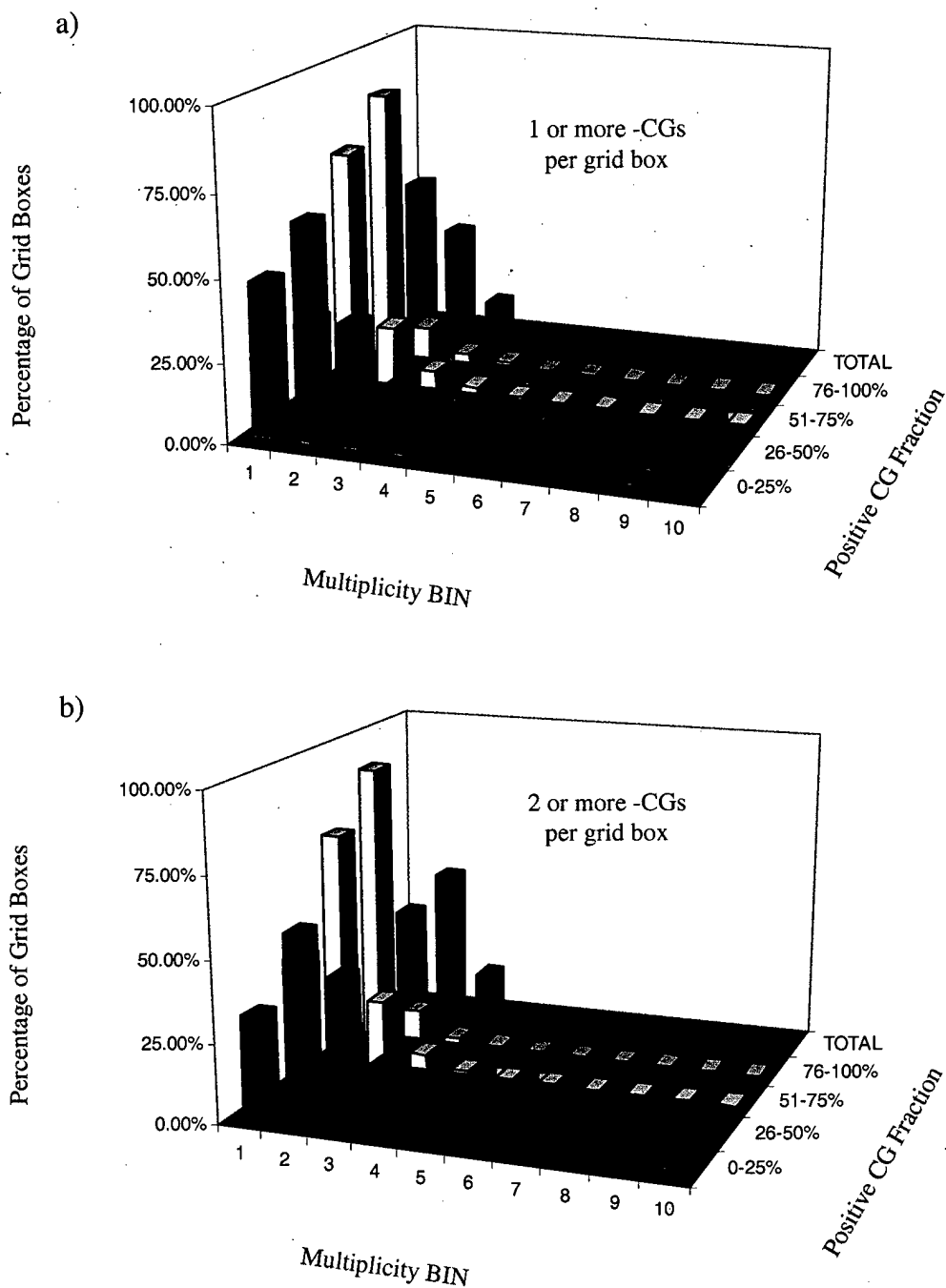
Figure 4.16: Normalized three-dimensional frequency distributions of average negative CG multiplicity as a function of positive CG fraction for grid boxes containing (a) one or more negative CGs per grid box and (b) two or more negative CGs per grid box.
