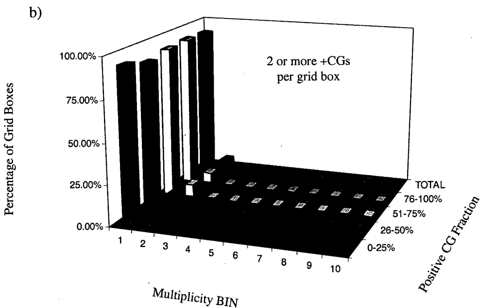
Figure 4.10: Normalized three-dimensional frequency distributions of average positive CG multiplicity as a function of positive CG fraction for grid boxes containing (a) one or more positive CGs per grid box and (b) two or more positive CGs per grid box.
