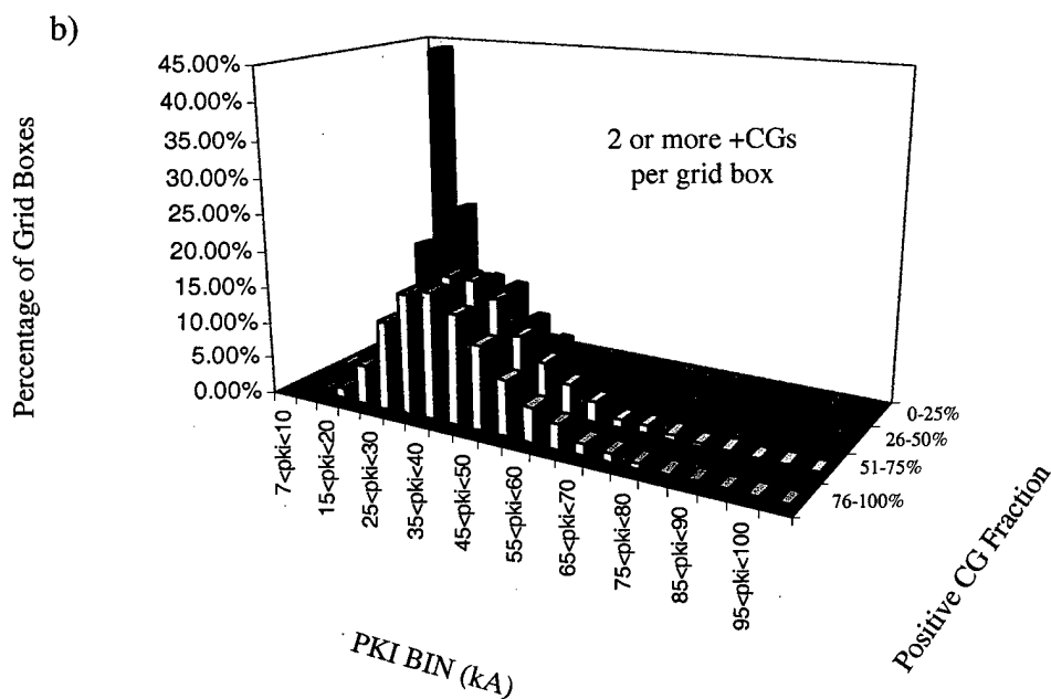
Figure 4.7: Normalized three-dimensional frequency distributions of average positive peak current as a function of positive CG fraction for grid boxes containing (a) one or more positive CGs per grid box and (b) two or more positive CGs per grid box.
