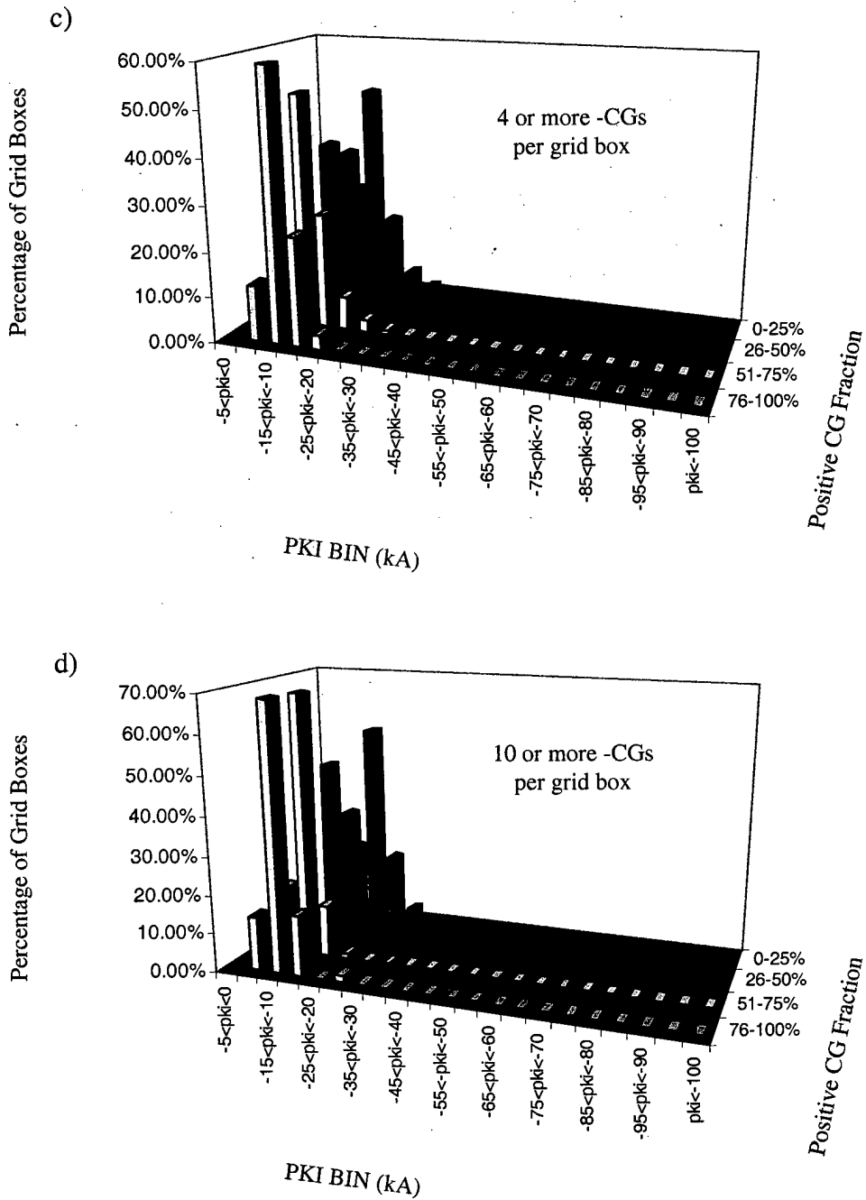
Figure 4.13: Normalized three-dimensional frequency distributions of average negative peak current as a function of positive CG fraction for grid boxes containing (c) four or more negative CGs per grid box and (d) ten or more negative CGs per grid box.
