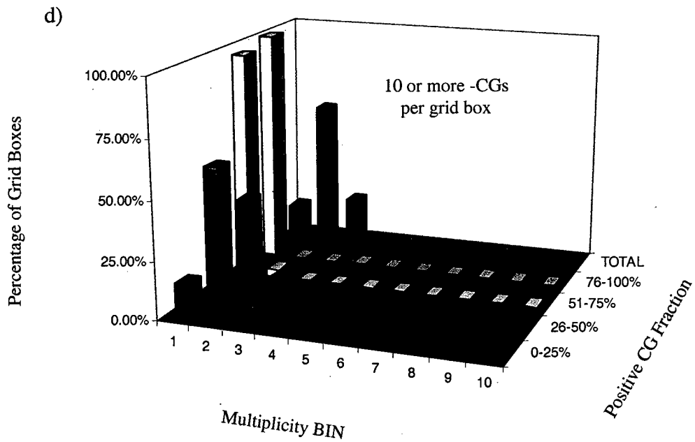
Figure 4.16: Normalized three-dimensional frequency distributions of average negative CG multiplicity as a function of positive CG fraction for grid boxes containing (c) four or more negative CGs per grid box and (d) ten or more negative CGs per grid box.
