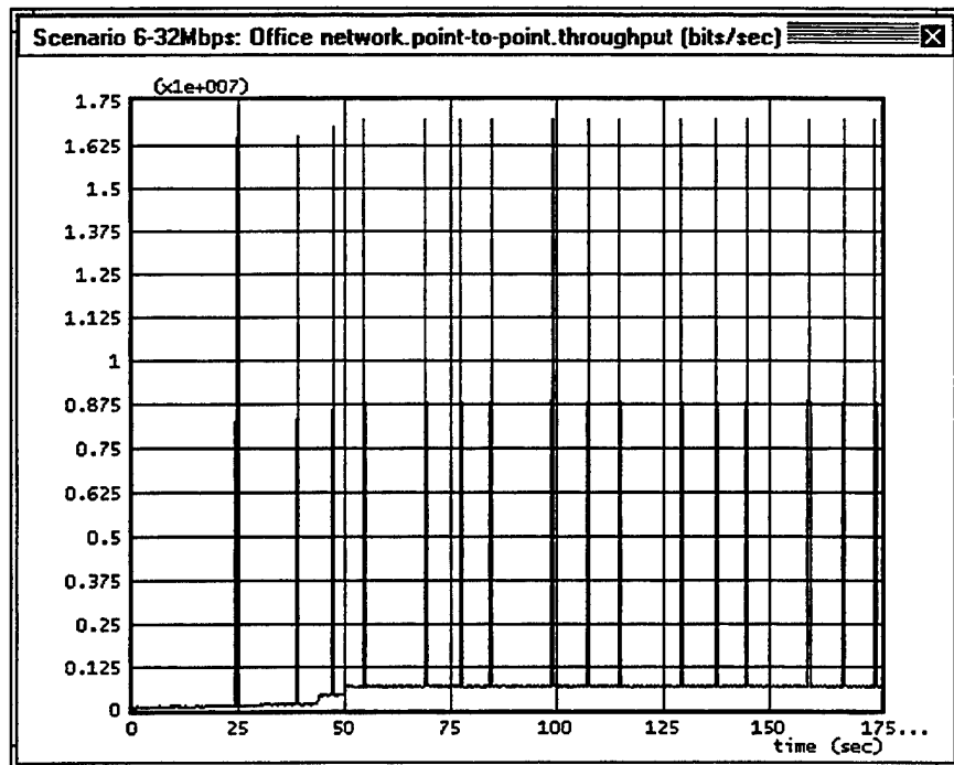
Figure 21. Data Throughput Simulation Results for Scenario 6.
