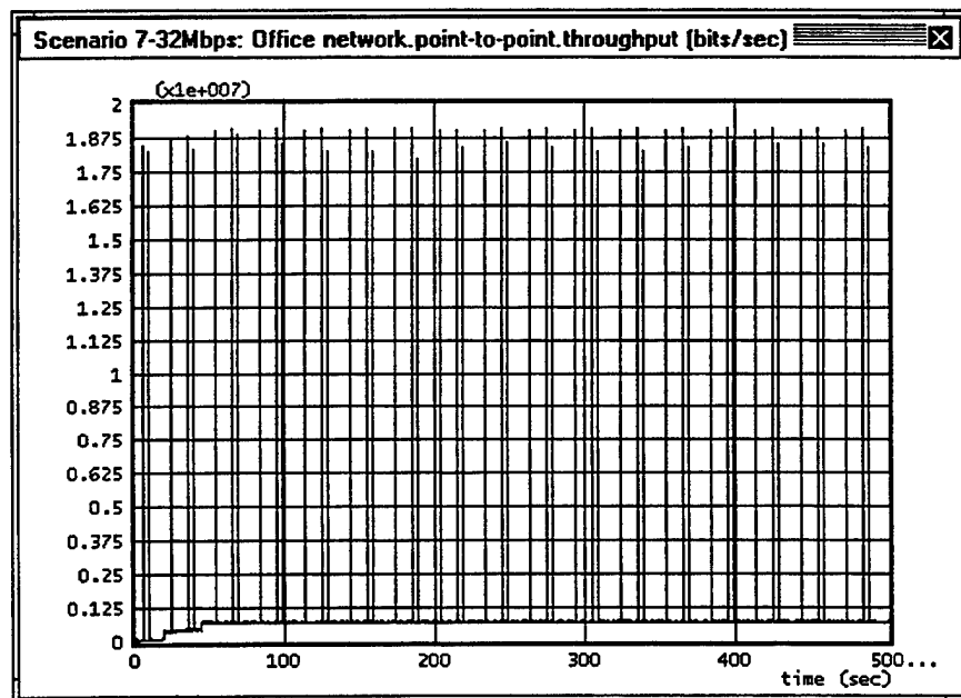
Figure 22. Data Throughput Simulation Results for Scenario 7.
