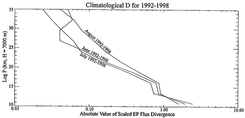
Figure 27. Composite of Figure 26 highlighting the decrease in negative D from June to July and subsequent increase in August in the lower half of the RMV (below ~25 km).
