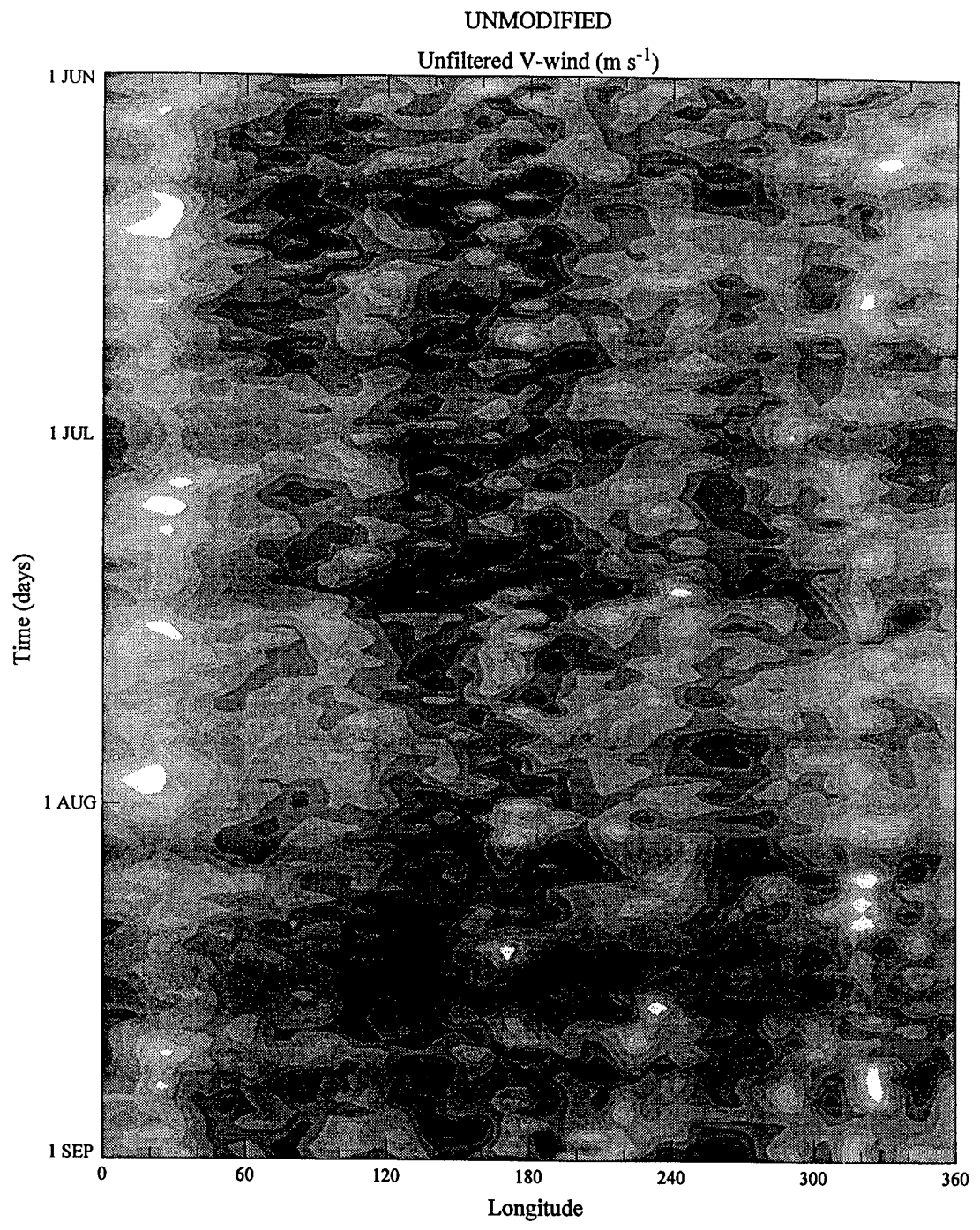
Figure 4. Hovmoller plot of the unmodified UKMO unfiltered meridional wind ( v ) for 1 June 1998 - 31 August 1998. Pressure level = 21.5 hPa, Latitude = 61.25°N.
