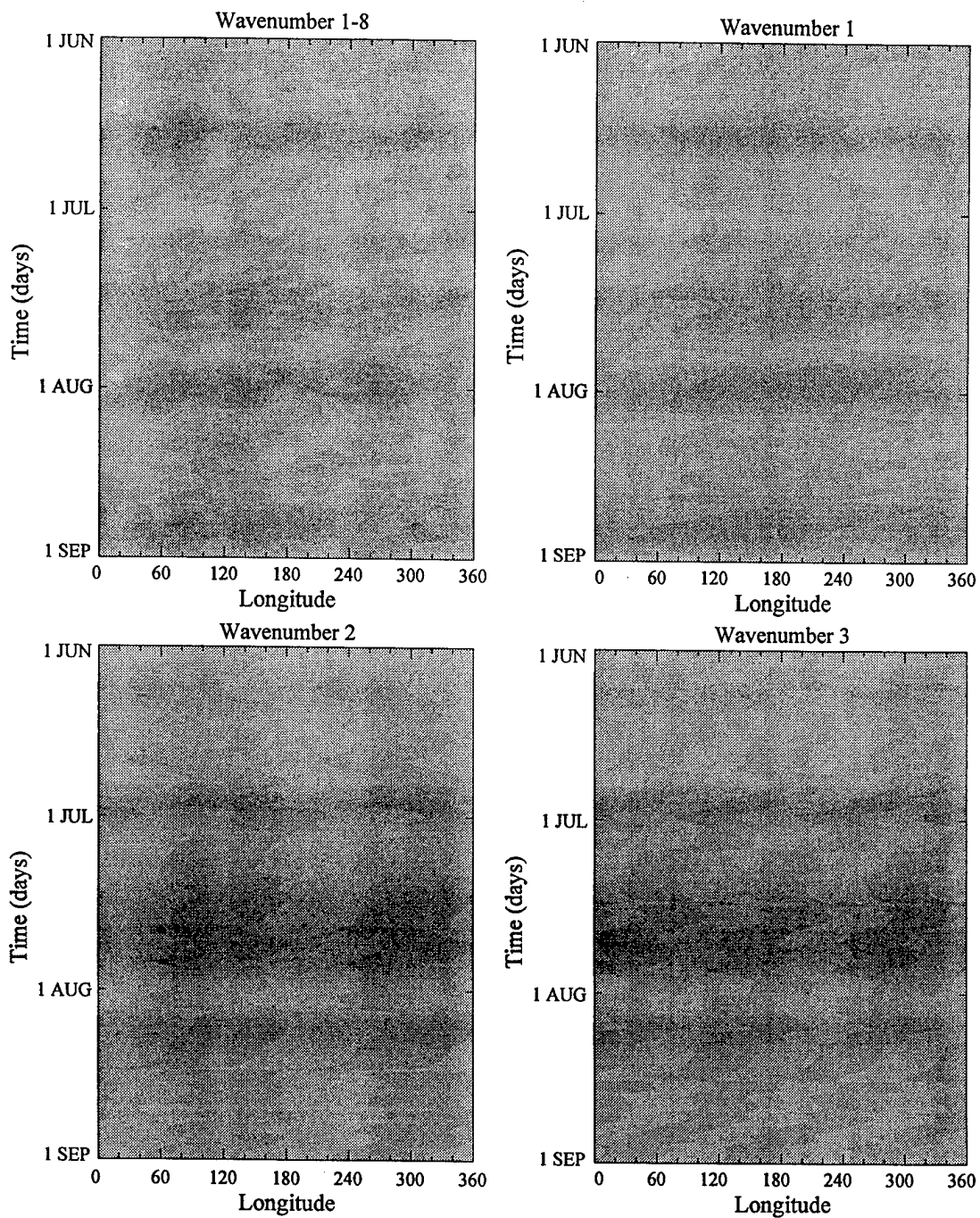
Figure 6. Hovmoller plots of the unmodified UKMO meridional wind ( v ) by zonal wavenumber for 1 June 1998 - 31 August 1998. Pressure level = 21.5 hPa, Latitude = 61.25°N.
