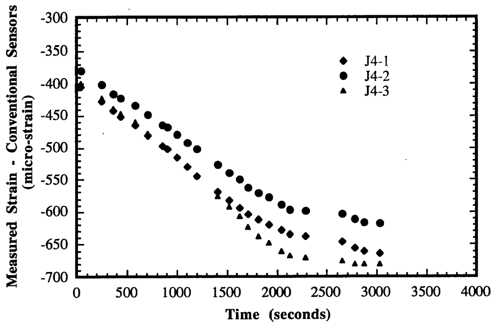
Figure 16. Strain data from conventional sensors located close to FBG array 1 during the same time frame as that of figure 15. Sensor J4-1 is close to the middle, J4-2 is close to the right and J4-3 is close to the left side of the floor (or flange ) of the box-girder.
