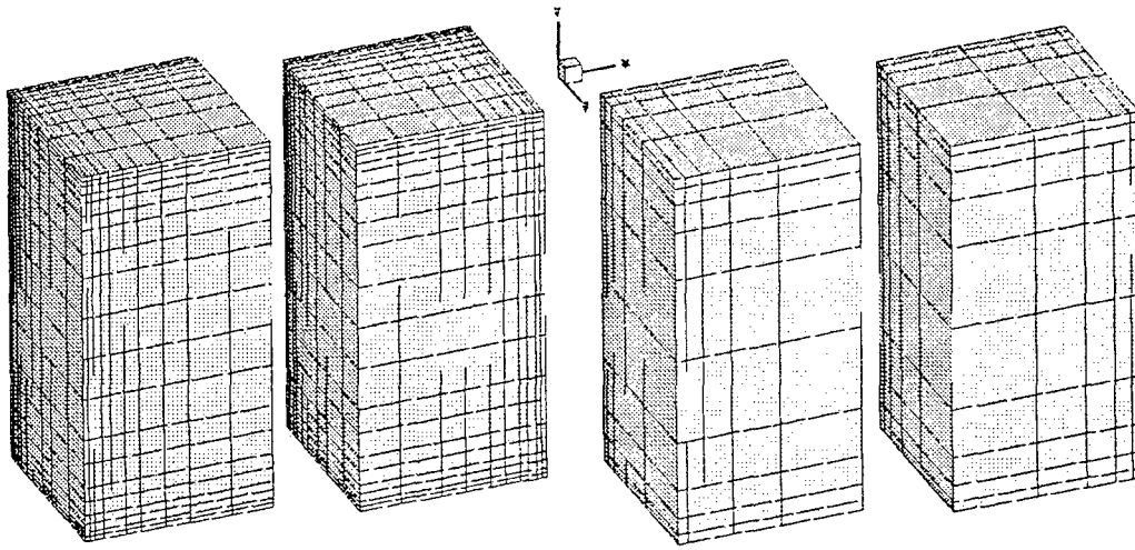
Figure 1. Computational mesh used for the two subdomain parallel solution of the lid-driven flow in a cubic cavity (left: 21 \times 21 \times 11 velocity, right: 11 \times 11 \times 6 pressure mesh).
