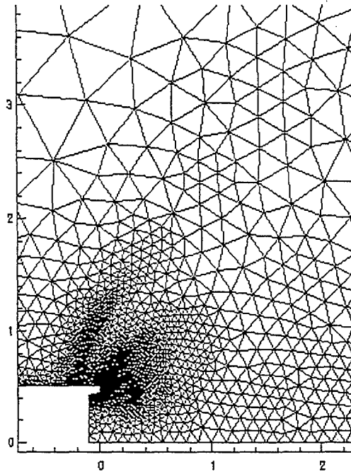
Figure 3 : adapted mesh around jet exit
