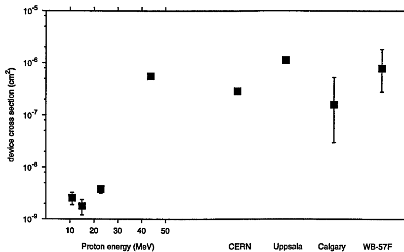
Figure 3: SEU cross section for the Dallas DS1650Y.70 SRAM measured for protons of different energy, for the CERF field at CERN, for a 180 MeV neutron beam at Uppsala, for a commercial flight from Frankfurt to Calgary and for WB-57F test flights.
