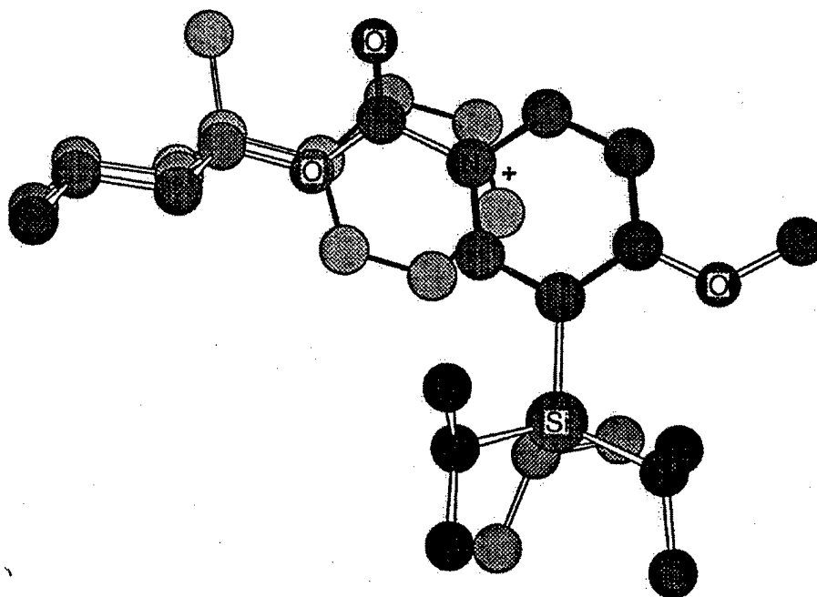
Figure 3: Rotamer B
