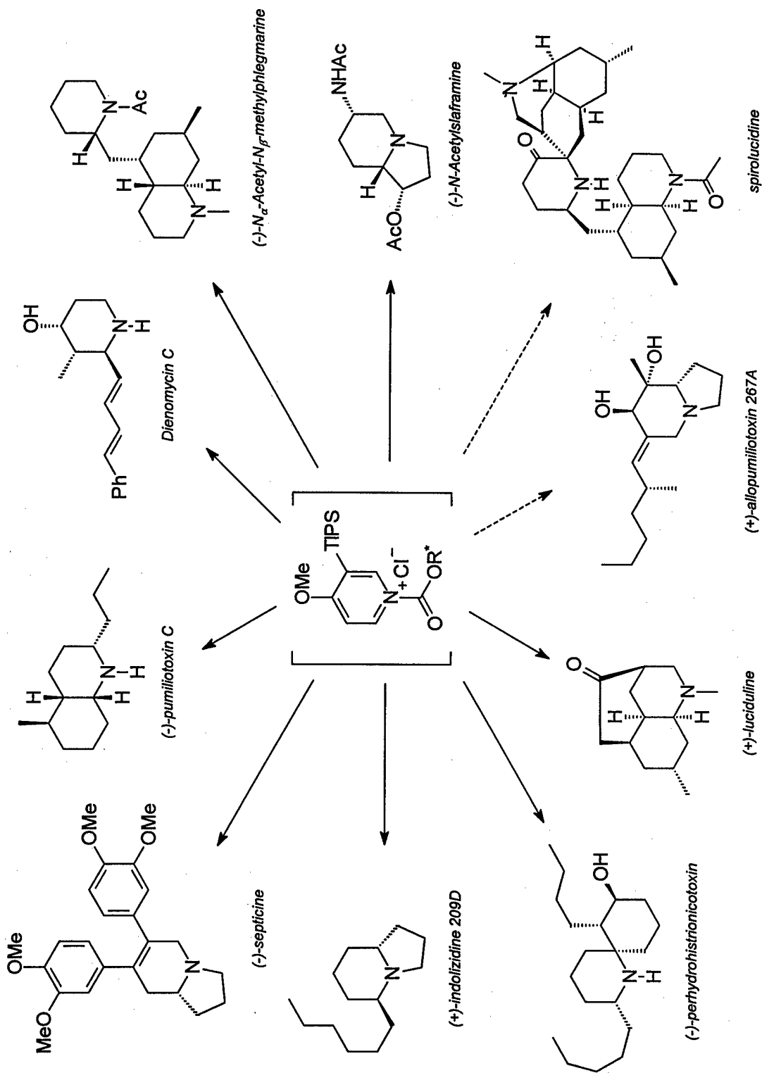
Figure 1: Past and Future Targets using Chiral N-Acyl-2,3-dihydro-4-pyridones
