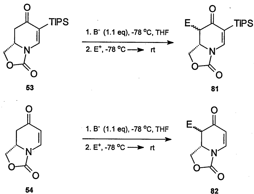
Scheme 16: Enolate Formation
