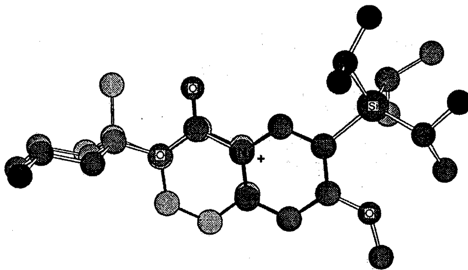
Figure 2: Rotamer A
