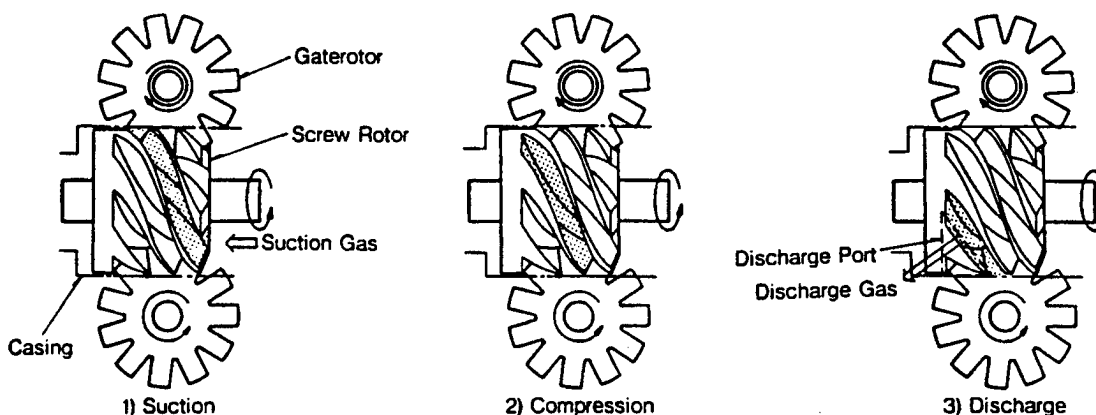
Figure C-5. Single Screw Compressor Sequence of Operation.
