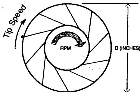
Figure D-9. Tip Speed.
