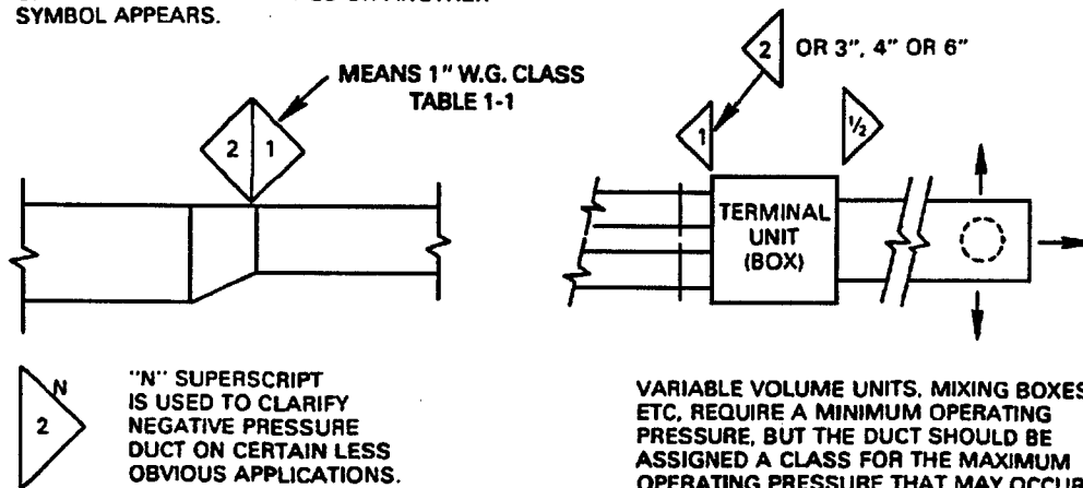
Figure D-28. Duct Pressure Class Designation.
