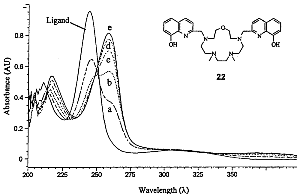
Figure 2. UV-visible spectra of free 22 and its Cu 2+ complexes in an aqueous buffered solution. [22] = 0.977 × 10 -5 M, [buffer] = 5.0 × 10 -2 M acetic acid (pH = 4.7). The labels a-e indicate 1-5 equiv of Cu 2+ added to the ligand successively.
