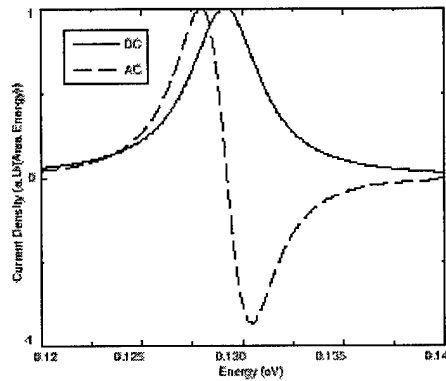
Figure 3. First order harmonics due to an AC perturbation on an RTD. DC component shows Loren lineshape as transmission of Figure 2b. AC component shows the principal value-type behavior to DC component.
