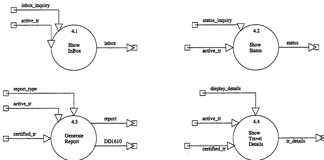
Figure 8. INQUIRIES process.
