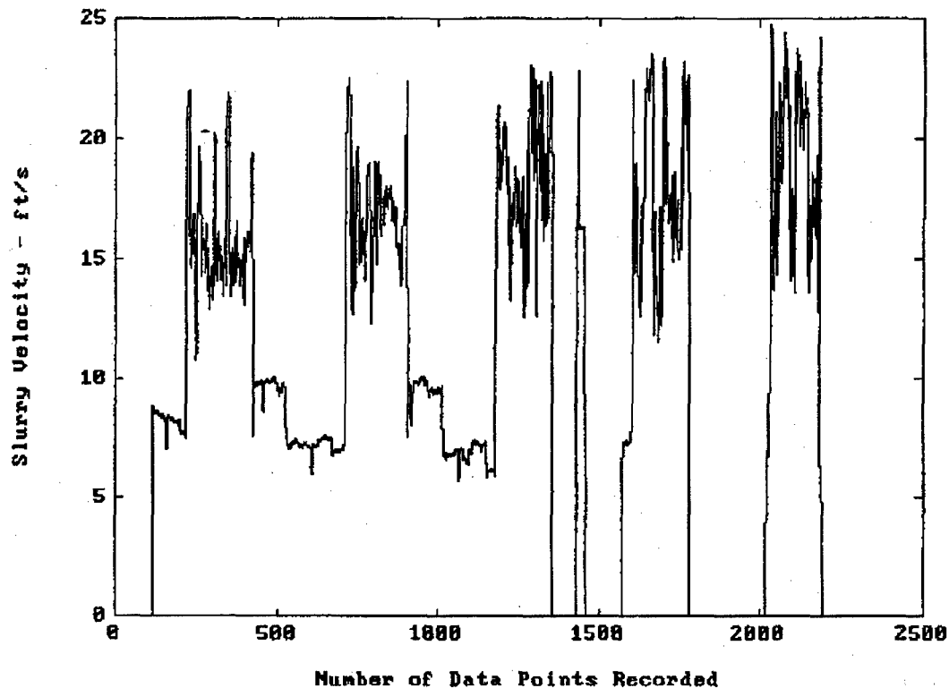
Figure 3. Slurry velocity data for the first five hopper loads
