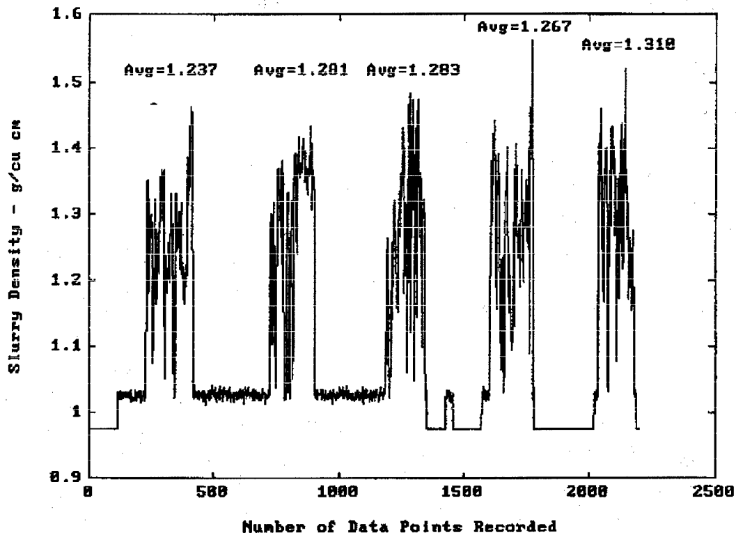
Figure 2. Slurry density data for the first five hopper loads
