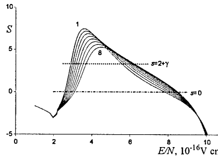
Fig. 4. Parameter s for transverse perturbations versus E/N in CO_2 at atmospheric pressure ( N=2.5 \times 10^{19} cm ^{-3} ). The numbers by the curves are the values of i in expression: j_b = 10 \times 2^{i-1} ( j_b in \mu A/cm^2 );
