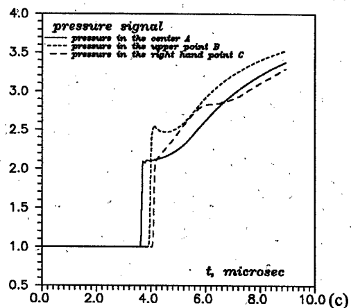
Fig.3. Initial temperature distribution (a); SW position at t=6\mu s (b); pressure signals from points A, B and C.
