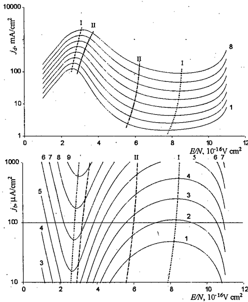
Fig.5. (a) Calculated current-voltage characteristics and (b) contour lines of the current density on the plane (j_b, E/N) for an NSSD in \text{CO}_2 at atmospheric pressure. The numbers by the current-voltage characteristics are the values of i in expression: j_b = 10 \times 2^{i-1} ( j_b in \mu\text{A}/\text{cm}^2 ); lines I and II are the boundaries of the acoustic-instability domains for transverse perturbations in isochoric and isobaric discharges, respectively the numbers by contour lines of the current density are the values of i in expression: j_b = 10 \times 2^{i-1} ( j_b in \text{mA}/\text{cm}^2 ).
