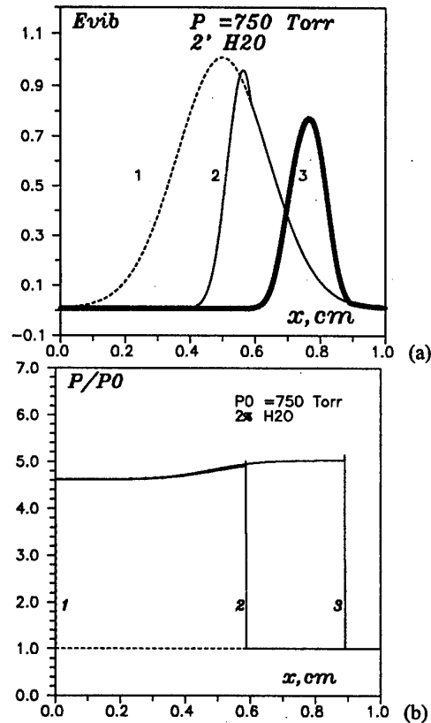
Fig.5. Profiles of vibrational energy (number of quanta per molecule) (a) and pressure (b) at P_0=750\text{Torr} at 3 time moments; 2% H_2O . Thin vibrational regions.
