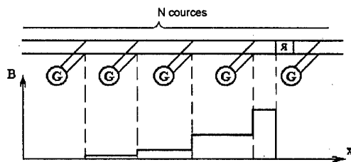
Fig. 6. The configuration of a distributed energy (current) input into the railgun barrel and the distribution of the magnetic field, B , over its length.
