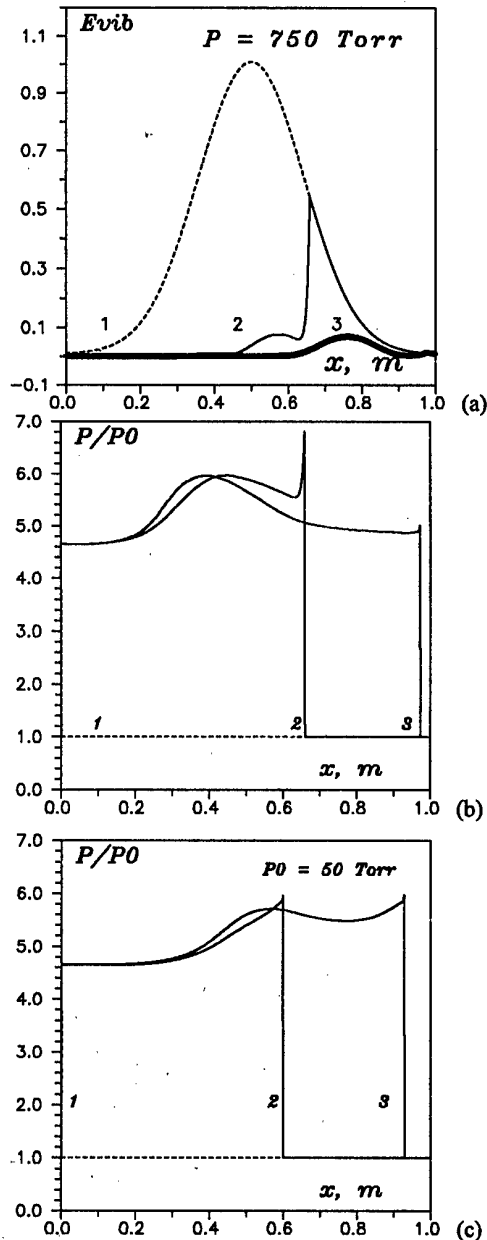
Fig.4. Profiles of vibrational energy (number of quanta per molecule) (a) and pressure (b) at P_0=750\text{Torr} , and also at P_0=50\text{Torr} (c) at 3 time moments; 1% H_2O .
