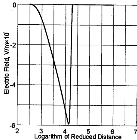
Fig.9. Electrical field [Td] vs logarithm of reduced distance \xi=\ln(12+x/\lambda) . Five component mixture, particle drift model case.
