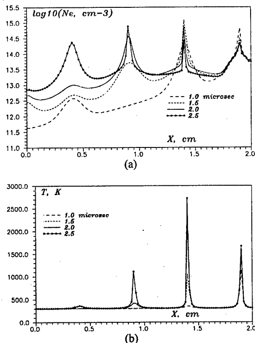
Fig.1. Distribution of electron number density (a) and gas temperature (b) at four successive time moments. Initial conditions are E_0/n=60\text{Td} , P=600\text{Torr} . Wave length of microwave radiation \lambda=2\text{cm} . Calculations have been performed for strong microwave fields using the discharge model proposed in [3].
