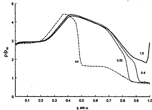
Fig.5. Density distribution in cross section of channel before the combustor of MPCE, M_\infty=6 , velocity pressure 3,7 \cdot 10^4 \text{ Pa} ; values for q/q_{cr} are indicated near the curves.
