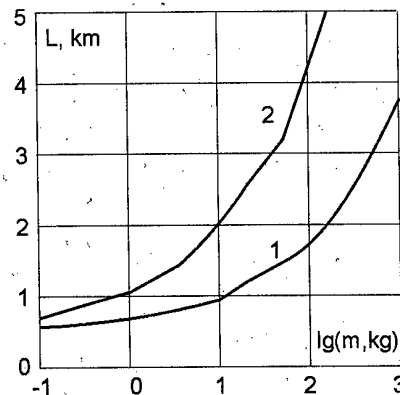
Fig. 2. Length of an accelerator required for the launch of payloads into geostationary orbit: 1 — L=5 ; 2 — L=20 .
