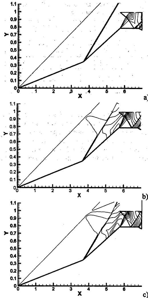
Fig.4. Density isolines for MHD controlled air intake at M_\infty=6 , velocity pressure 3,7 \cdot 10^4 \text{ Pa} , B=3 \text{ Tesla} a) q/q_{cr}=0 ; b) q/q_{cr}=0,02 ; c) q/q_{cr}=1,0 ;
