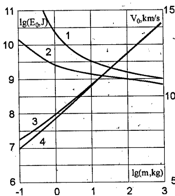
Fig. 1. Muzzle velocity (1,2) and kinetic energy (3,4), required for the launch of payloads into geostationary orbit: 1, 3 — L=5 ; 2, 4 — L=20 .
