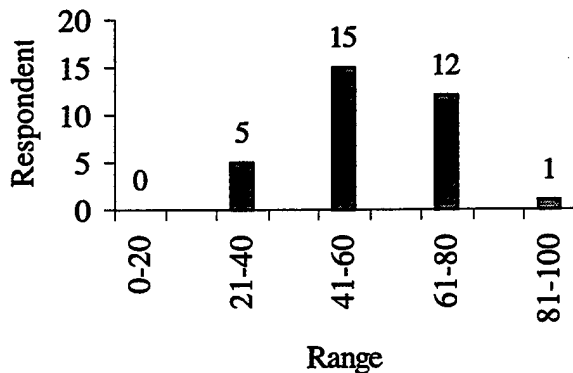
Figure 4.13 CDI (Turkish)
