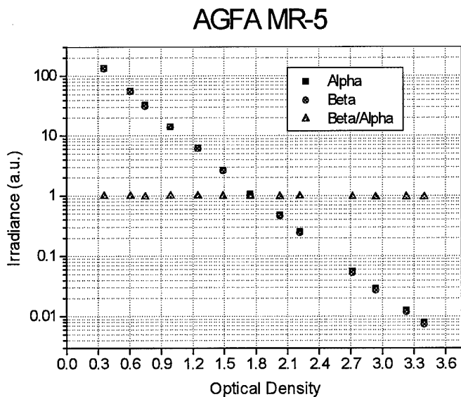
Figure 22. Plot of the Mueller matrix elements m_{11} (=alpha, \alpha ), m_{22} (=beta, \beta ), and the ratio of m_{22}/m_{11} (= \beta/\alpha ) versus optical density for Agfa MR 5 mammography film.
