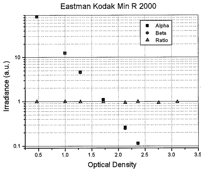
Figure 24. Plot of the Mueller matrix elements m_{11} ( = \alpha ), m_{22} ( = \beta ), and the ratio of m_{22}/m_{11} ( = \beta/\alpha ) versus optical density for Kodak Min R 2000 mammography film.
