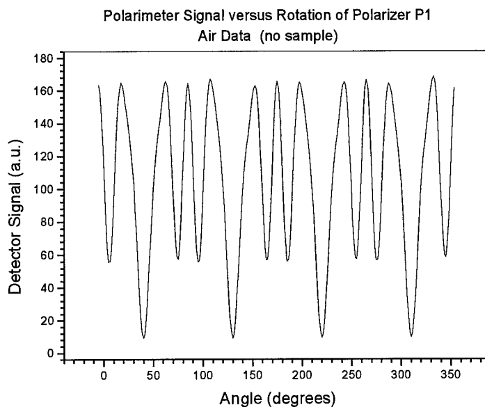
Figure 7. Plot of air data acquired with polarimeter. Air data was acquired each day that mammography film samples were analyzed.
