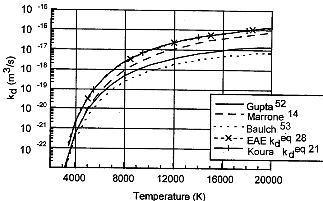
Figure 4 Rate Constants for Dissociation of O 2 by Argon
