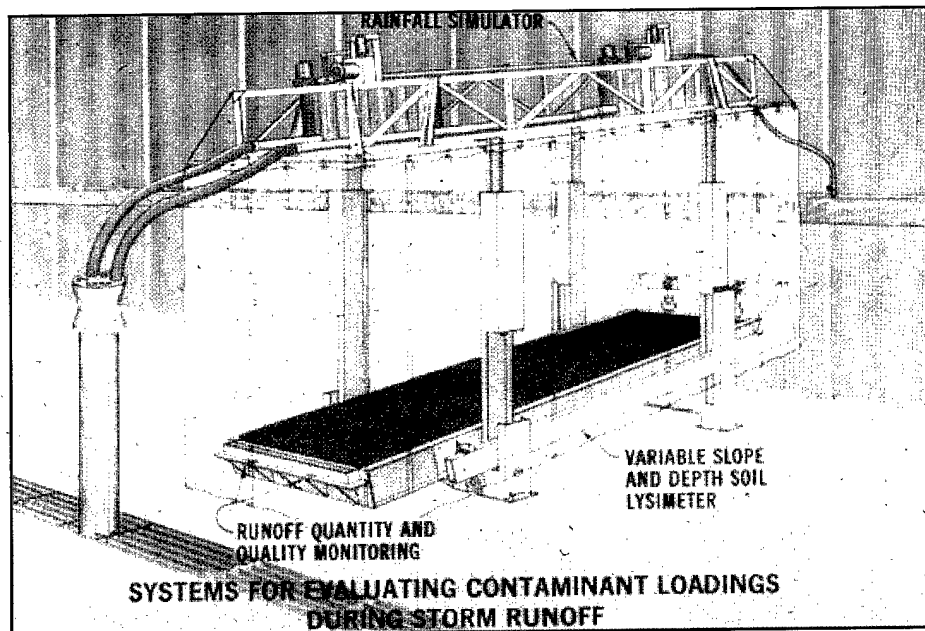
Figure 1. Schematic of the rainfall simulator lysimeter system
