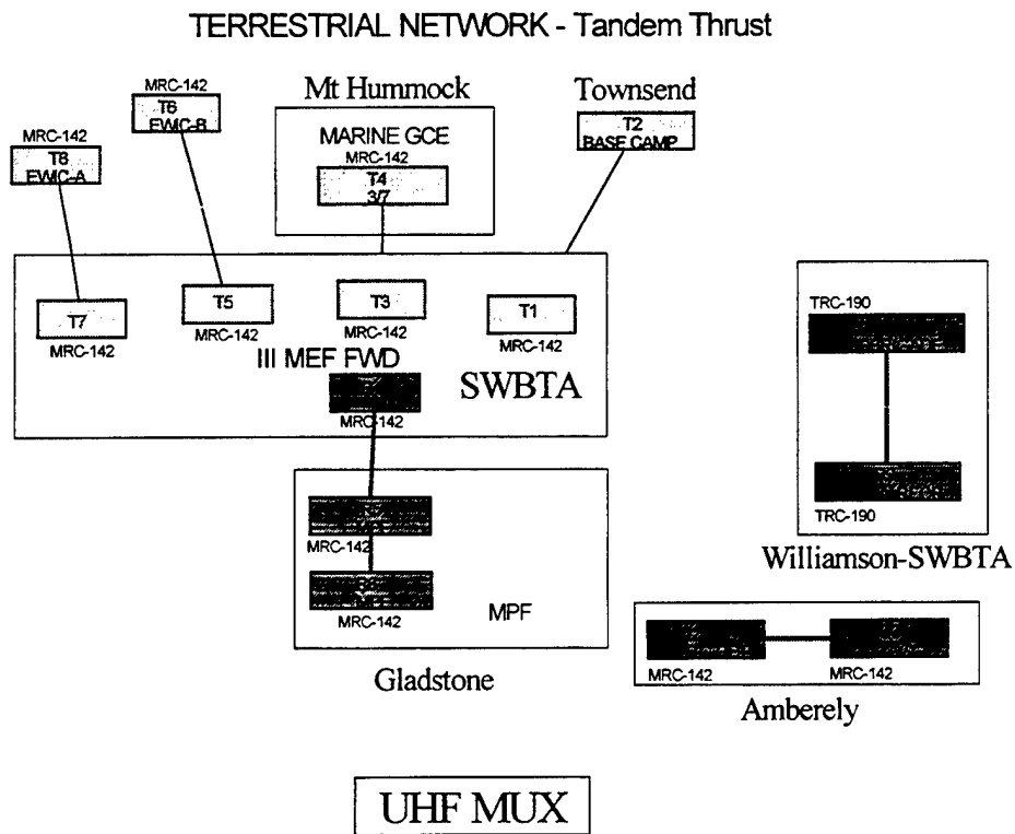
Figure 7 UHF Terrestrial Multichannel Diagram Tandem Thrust 97
