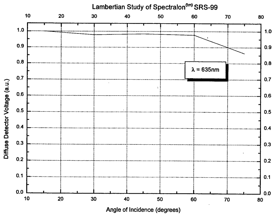
Figure 6. Lambertian Study of Spectralon TM SRS-99.
