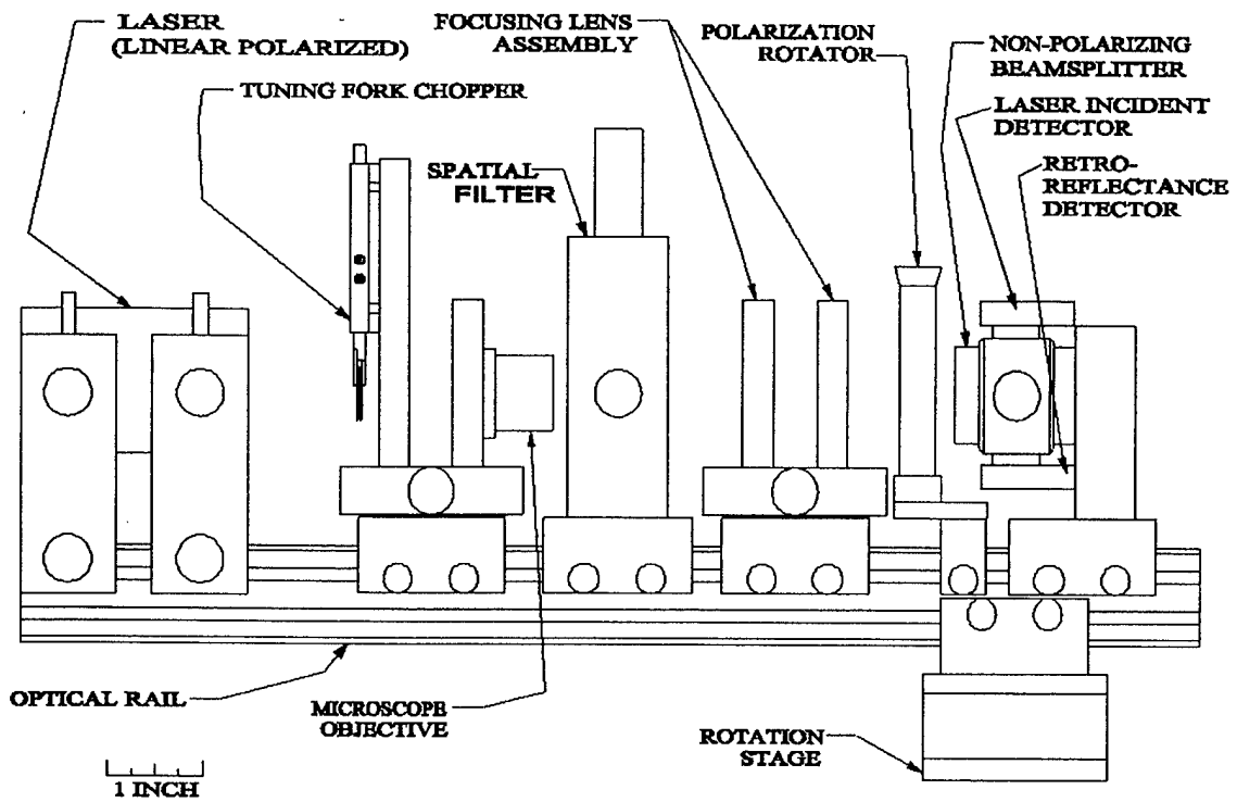
Figure 3. Laser Section.
