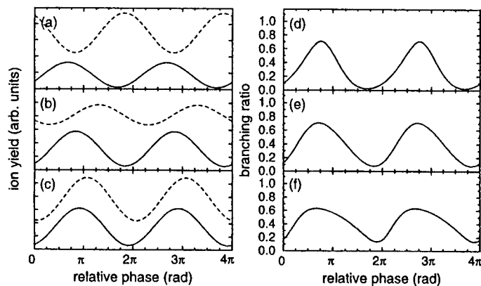
Figure 4: Modulation of the photoionization signals for \text{Xe}^+ 5p^5 2P_{3/2} (solid) and 2P_{1/2} (dashed) ion at three different final state energies (a) 123000\text{cm}^{-1} , (b) 125100\text{cm}^{-1} , and (c) 127100\text{cm}^{-1} above the atomic ground state as a function of the relative phase \phi . The laser intensities are chosen to be I_{3\omega} = 10\text{W}/\text{cm}^2 and I_{\omega} = 10^{10}\text{W}/\text{cm}^2 . (d)-(f) Branching ratios as a function of the relative phase \phi . Graphs (d)-(f) correspond to graphs (a)-(c), respectively.
