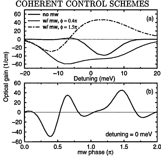
Figure 6. Optical gain with and without a mw driving field, for a short probe pulse (200 fs) in a closed system. (a) shows the optical gain profile's dependence on the mw field and its phase, while (b) shows the mw phase dependence of optical gain at a certain detuning (0 meV). As shown, the optical absorption is sensitive to the phase of the mw field.
