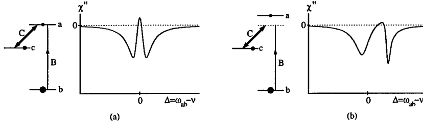
Figure 2. (a) Gain can be produced even when N_b is larger than N_a and N_c . When level |a\rangle is “detuned”, as indicated in (b), a larger Rabi-frequency C is required to obtain LWI and gain is reduced due to “Stark broadening” (power broadening) of level |a\rangle .
