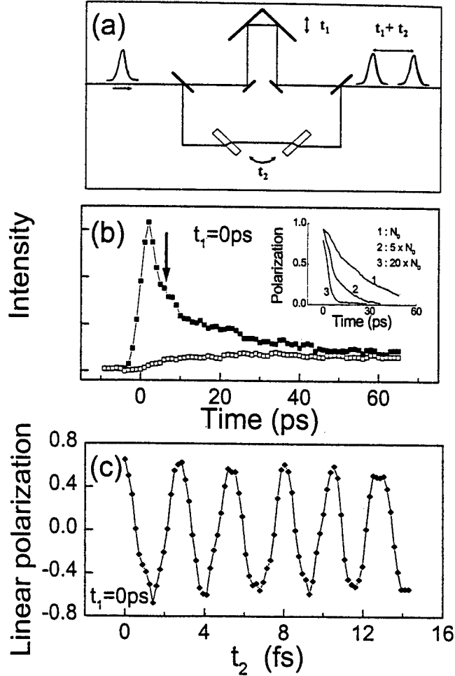
Figure 1. (a) Schematic excitation arrangement. In (b) and (c) the sequence configuration is (\sigma^+, \sigma^-) and t_1 = 0 . (b) The time evolution of P' (■) and P'' (□) for t_2 = m\lambda/c . Inset: dependence of the linear polarization decay (characteristic time T_{2z} ) as a function of the photocreated exciton density, N_0 \approx 10^9 \text{ cm}^{-2} . (c) Linear polarization P' , measured 4 ps after the excitation [arrows in (b)], as a function of the fine temporal separation t_2 between the two excitation pulses.
