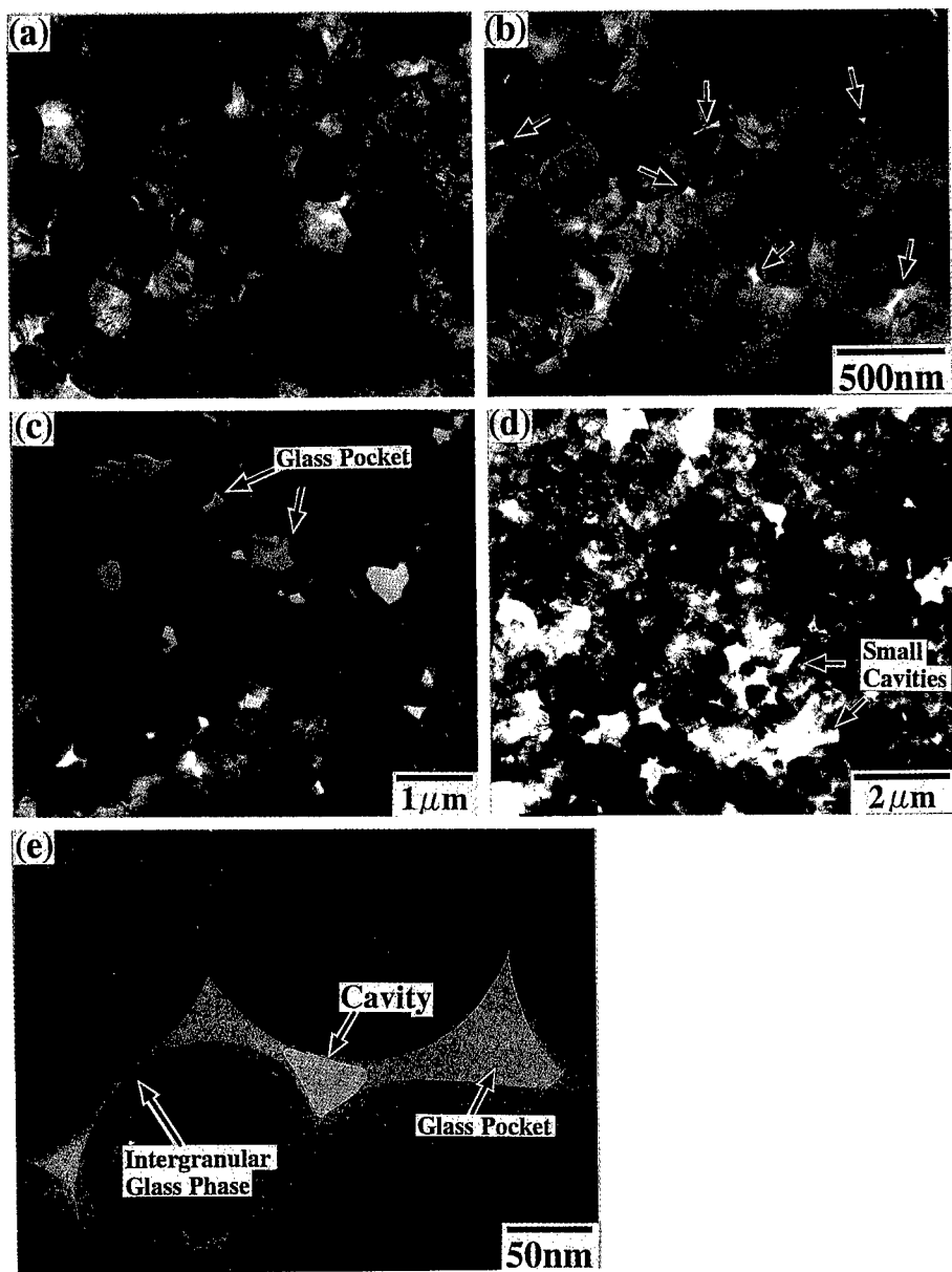
Fig. 4 Bright field TEM micrographs of the 0.3-wt%-SiO 2 -doped 3Y-TZP with initial grain sizes of 0.27 and 0.4 \mu m. (a) and (b) are undeformed, and (c) through (e) are deformed to failure. Nanometer-sized glass pockets are indicated with arrows. (e) also shows a cavity nucleus in the precipitated glass phase.
