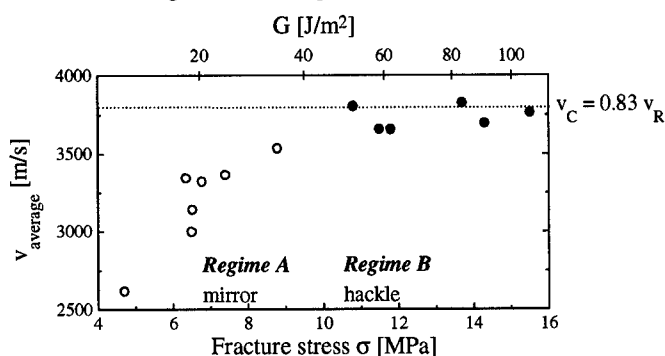
Fig. 3: Average crack velocity for the (110)[\bar{1}\bar{1}0] crack system as a function of the far-field stress at the onset of fracture. An increase of the velocity at lower stresses is followed by a regime where the velocity curve saturates. The generated fracture surface is smooth and mirror-like over the whole crack path (open circles) for the lower stresses. At high stresses a transition from mirror to hackle zones is observed along the crack propagation direction (solid circles).
