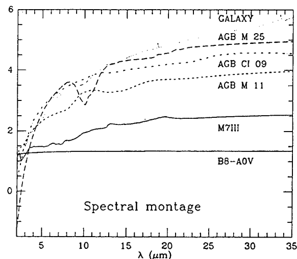
FIG. 3. Montage of intrinsic templates.
