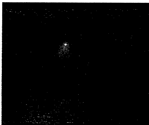
Figure 2b. Hyakutake in MSX Band C.
