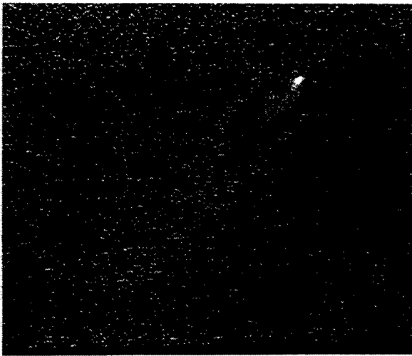
Figure 4b. Tabur in MSX Band C.
