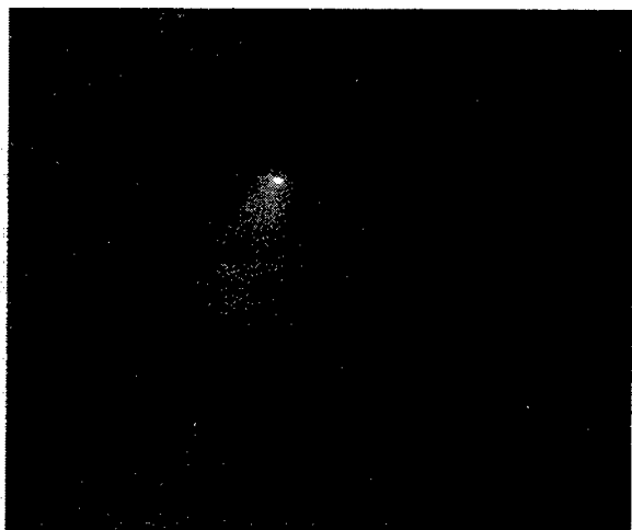
Figure 2a. Hyakutake in MSX Band A.
