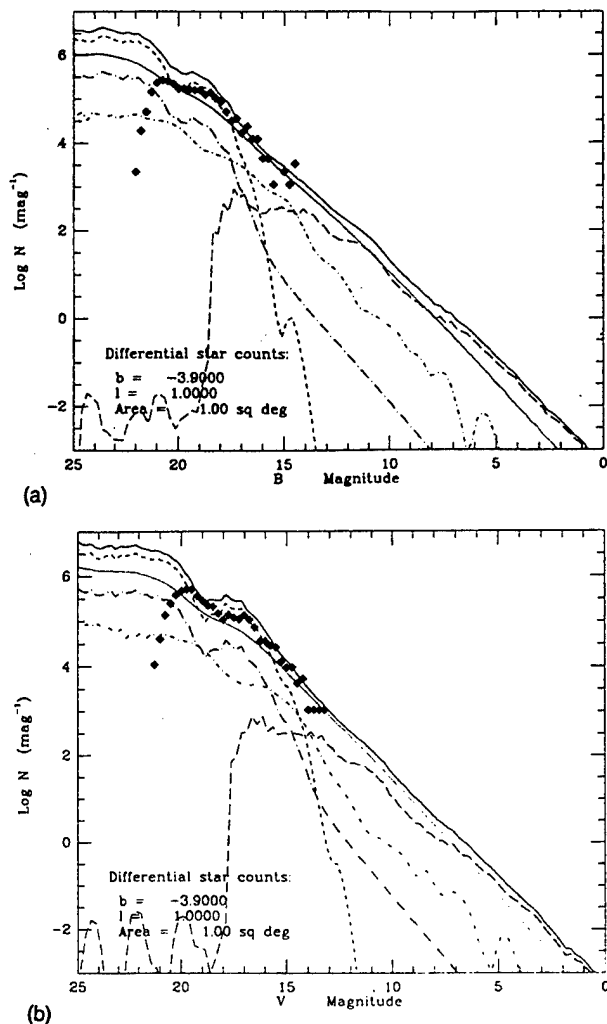
FIG. 4. Performance at B and V illustrated by Terndrup's (1988) differential counts for Baade's Window (filled diamonds). Lines as in Fig. 1, with the addition of: short dashes, bulge; short dash-dot, molecular ring. (a) B . (b) V . Note the incompleteness of the observed counts fainter than 16th magnitude.
