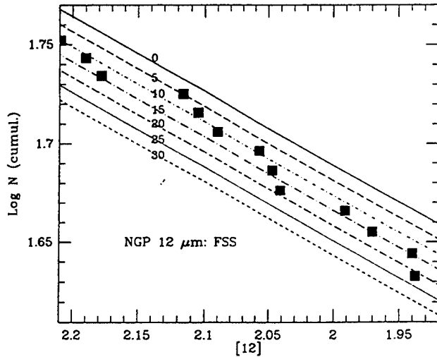
FIG. 3.—Cumulative IRAS counts for the NGP at 12 \mu\text{m} from the FSS (filled squares), boosted by a factor of 1.130 to allow for the area unobserved by IRAS . The curves represent SKY predictions for z_0 = 0\text{--}30 pc in 5 pc steps, as labeled. To illustrate the separation of these curves, the detail is shown for the middle of the useful range of IRAS data.
