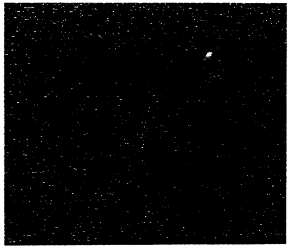
Figure 4d. Tabur in MSX Band E.
