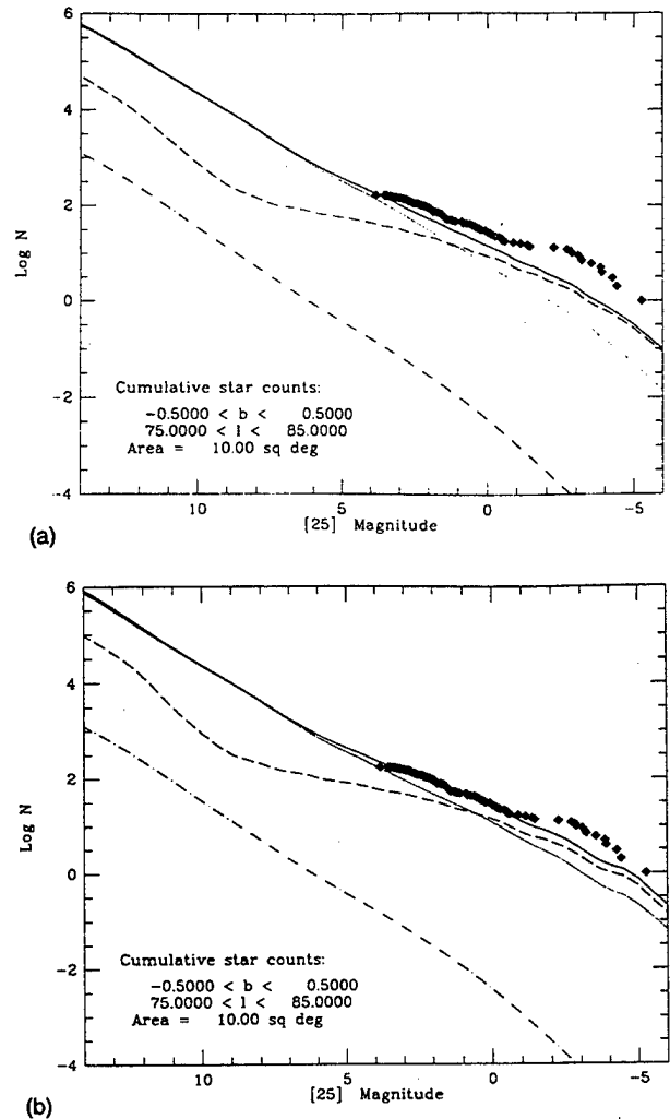
FIG. 1. Typical improvements achieved by the new model compared with WCVWS' first version. 25 \mu\text{m} predictions for the zone -0.5 < b < 0.5 , 75 < l < 85 . Diamonds, observed counts; solid line, total model prediction; dots, disk; long dashes, spiral arms, spurs, and Gould's Belt; long dash-dot, halo. (a) WCVWS. (b) New model.
