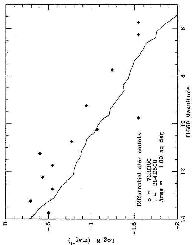
FIG. 1.—Comparison between SKY's predicted differential counts and those measured by FAUST. In this and subsequent figures, diamonds represent observed counts; solid line, total model prediction; dots, disk (often indistinguishable from the solid line); long dashes, arms; short dash-dot, molecular ring. Each figure is labeled with the Galactic coordinates of the center of the fully sampled FAUST field. (a) field 2; (b) field 5; (c) field 8; (d) field 9; (e) field 10; (f) field 11; (g) field 13; (h) field 14; (i) field 15; (j) field 16; (k) field 17; (l) field 18.
