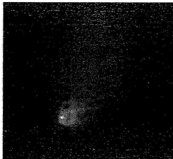
Figure 1c. Hale-Bopp in MSX Band D.
