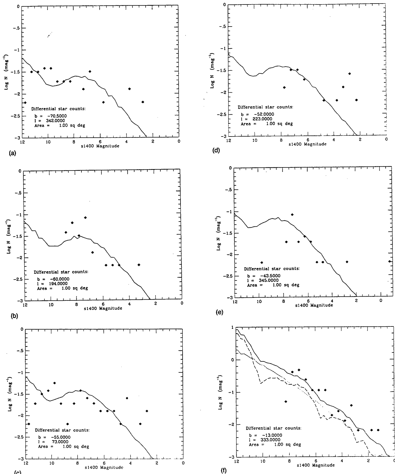
FIG. 5. Comparison of predictions and observed differential starcounts at 1400A for the target fields of the S201 experiment. All models represent the default ultraviolet mode, without extra populations or extra associated extinction in the local spurs. (a) Grus; (b) Cetus; (c) Aquarius; (d) Fornax; (e) Pavo; (f) Norma; (g) Sagittarius; (h) Cygnus. Diamonds: observations. Line styles as in Fig. 1.
